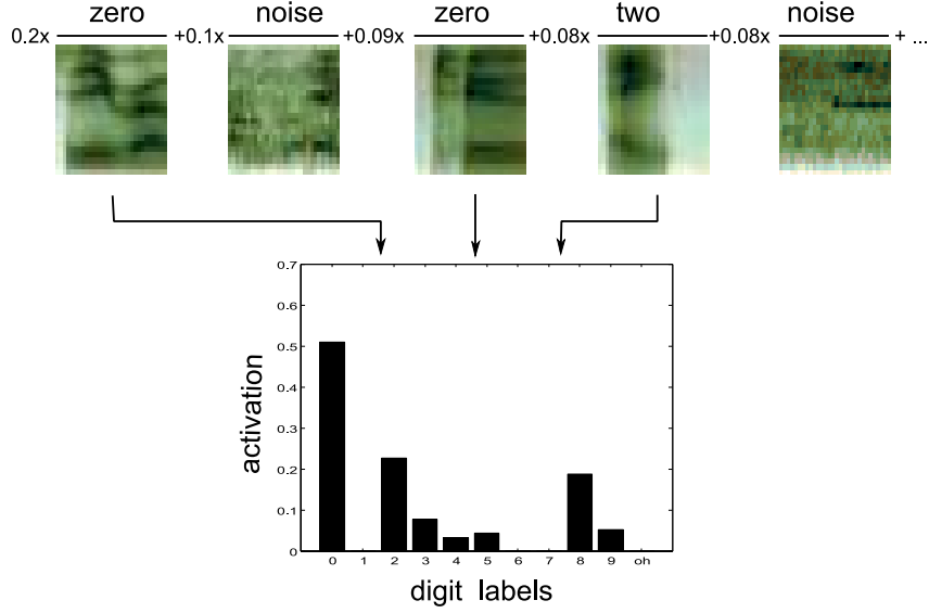
Fig. 8. By associating each dictionary atom of Fig. 5 with a word label, the linear combination of speech atoms in Fig. 5 serves directly as evidence for the underlying word classes. We observe that the word “zero”, underlying the noisy observation of Fig. 5, does indeed obtain the highest score.
