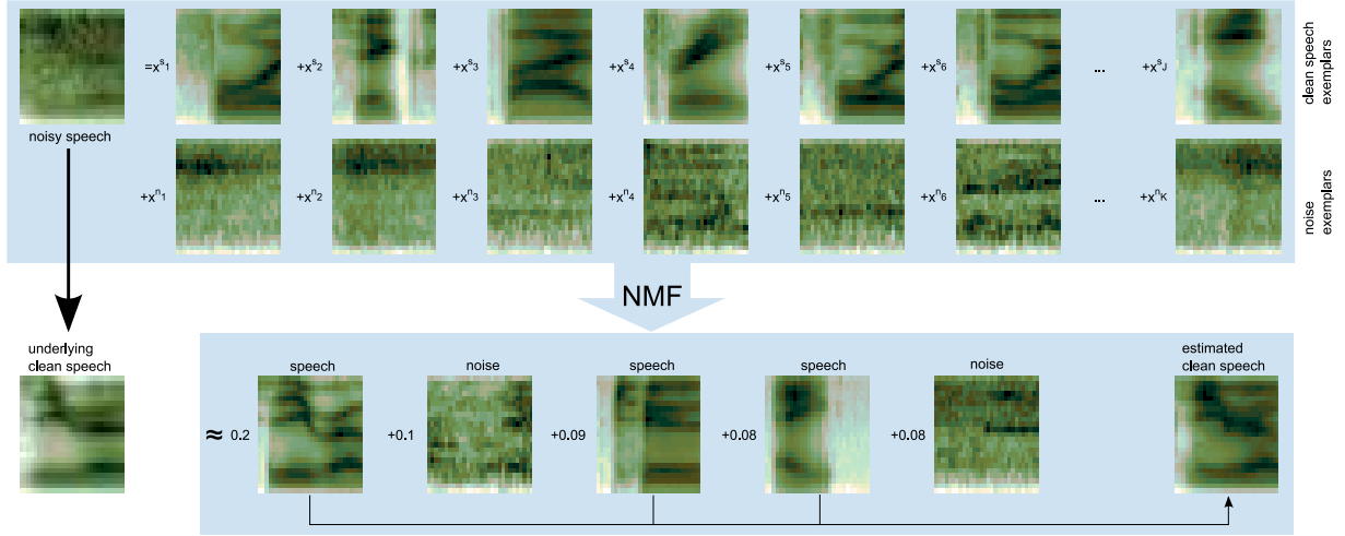
Fig. 5. An example of supervised separation of noisy speech. In the top left corner, we display the noisy spectrogram of the isolated word “zero”, corrupted with babble noise. In the top panel, we display parts of the speech and noise exemplar dictionaries. In the bottom panel, the five atoms with the highest weight are shown. The bottom left spectrogram illustrates the underlying clean speech, whereas the bottom right spectrogram shows the clean speech reconstruction.
