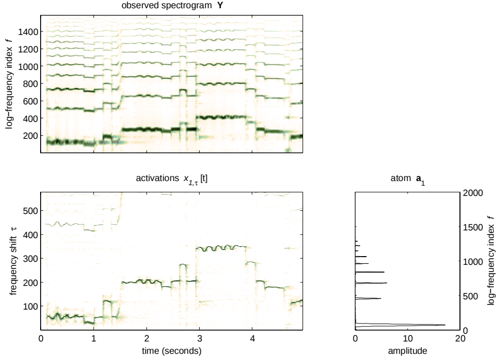
Fig. 13. Illustration of non-negative matrix deconvolution in frequency. A spectrogram of a violin passage with a logarithmic frequency resolution (upper panel) has been decomposed into a weighted sum of shifted versions of a single harmonic atom vector (bottom right panel). The activations for each pitch shift and each frame are illustrated on the bottom left panel. The model allows representing notes of different pitches with a single harmonic spectrum that is shifted in frequency.
