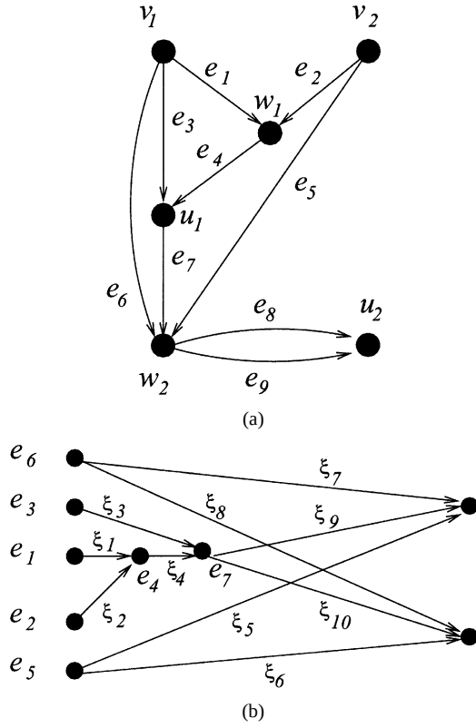
Fig. 5. (a) Network with two source and two sink nodes. (b) Corresponding labeled line graph.
