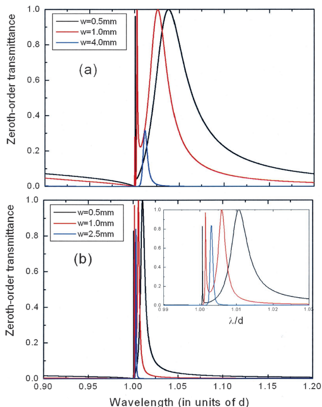
Fig. 2. Theoretical zeroth-order transmittance spectra corresponding to different infinite hole arrays with (a) R = 1.25 mm and (b) R = 1 mm. The inset in (b) represents the same physical quantity but for a smaller range of wavelengths.
