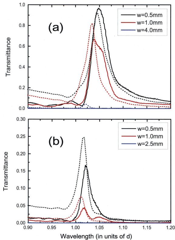
Fig. 3. Experimental transmittance spectra (solid curves) and theoretical total transmittance curves (dashed curves) for the 31 \times 31 arrays corresponding to the same geometric parameters as in Fig. 2. Different hole arrays with (a) R = 1.25 mm and (b) R = 1 mm are analyzed.
