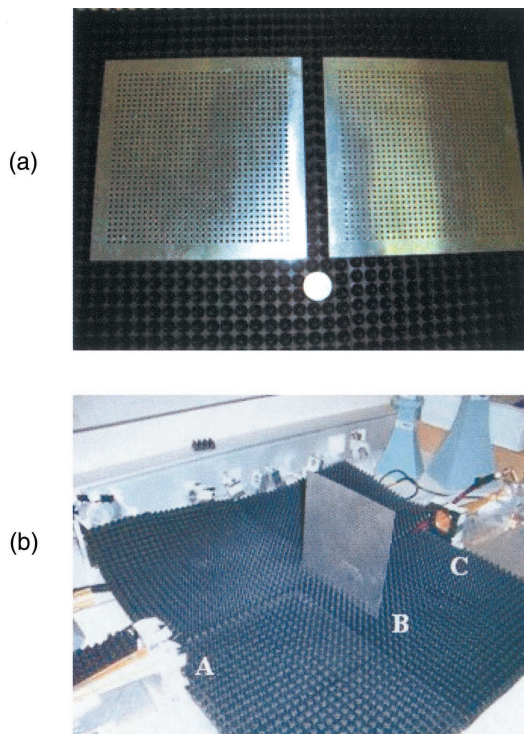
Fig. 1. (a) Photographs of two of the six samples analyzed in the experiment (left, R = 1.25 mm, w = 0.5 mm; right, R = 1 mm, w = 0.5 mm). (b) Photograph of the experimental setup: A, corrugated horn antenna acting as source of millimeter waves; B, sample; C, receptor antenna.
