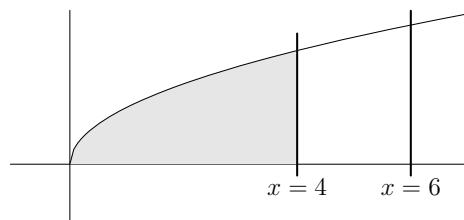
Figure 1: Region to be revolved.
