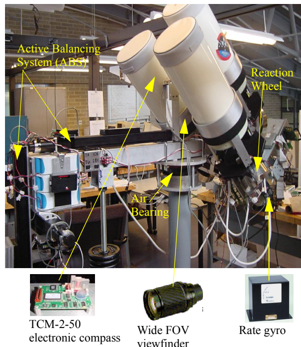
FIG. 2: The final ARGOS system with the three ACS sensors shown in the bottom
