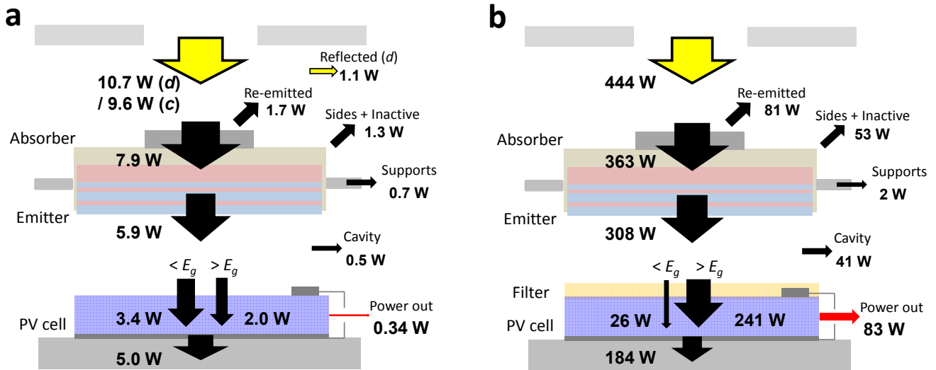
Supplementary Fig. 5 | Power conversion and loss mechanisms at an irradiance of 75 \text{ W/cm}^2 in the following NARO-STPVs (obtained using the SQIDD): a , the experimentally demonstrated AR=7 ( 1 \text{ cm}^2 ) device ( d and c represent diffuse and collimated irradiance, respectively); and b , a scaled-up ( 100 \text{ cm}^2 ) AR=17 device utilizing a high-quality 0.55 \text{ eV} PV module with a sub-bandgap reflector 6 . The scaled-up device was simulated with 1 \text{ mm} gaps between the shield/absorber and emitter/PV, and mounted using 8 stainless steel supports (difference between the diffuse and collimated irradiance is negligible in this configuration). Width of arrow is proportional to the magnitude of power it represents.
