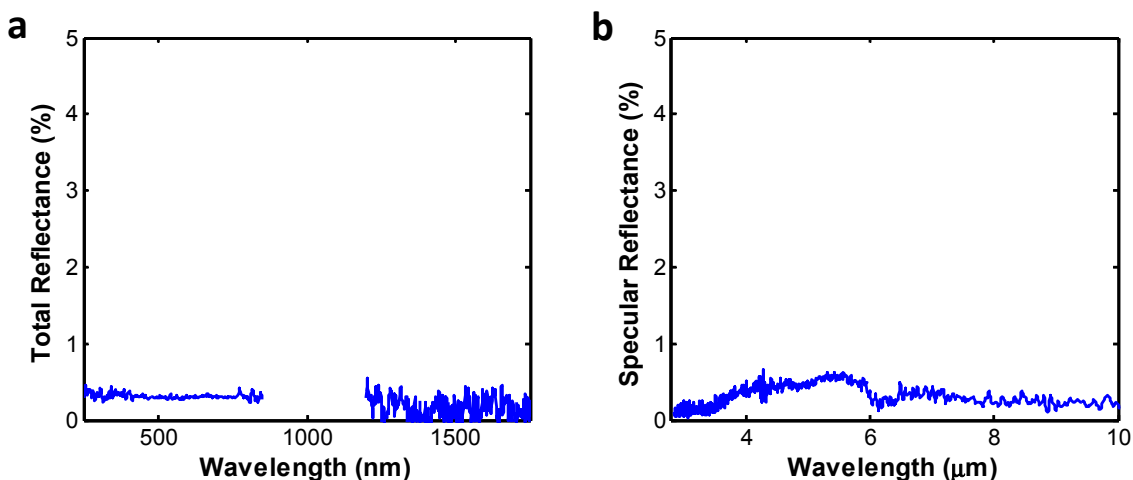
Supplementary Fig. 1 | Optical characterization of MWCNT absorber. a , Total reflectance (diffuse + specular) spanning the relevant solar wavelength range (0.25-1.75 \mu\text{m} ); data near 1 \mu\text{m} omitted due to high noise level associated with lamp/detector change. b , Specular reflectance (30° incident angle) in the infrared (2.8-10 \mu\text{m} ).
