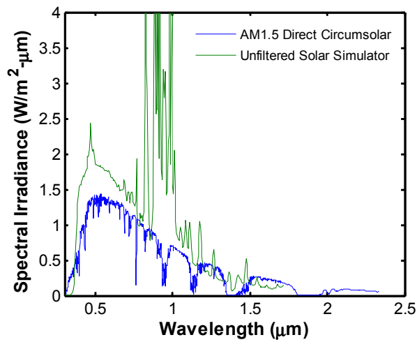
Supplementary Fig. 3 | Simulated solar spectrum. Comparison between the AM1.5 direct spectrum used a standard for CSP applications and the spectrum provided by the Xe-arc lamp in our experiments.
