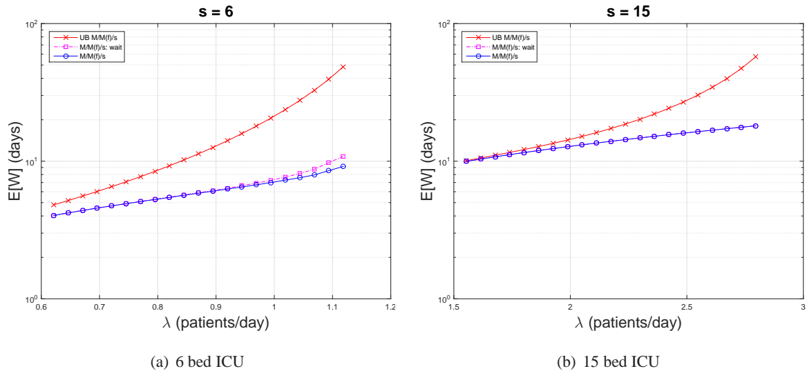
Figure 8 Simulation of M/M(f)/s system with a delay effect that is wait (not number of jobs in system) dependent.
