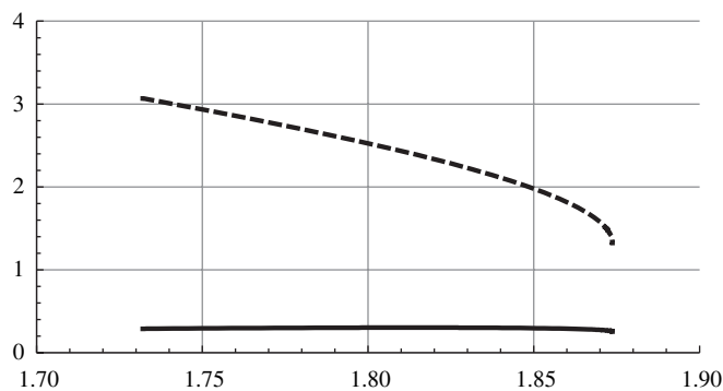
Figure 8. S -dependence of the parameters \tilde{A} (solid line) and \tilde{B} (dashed line).
