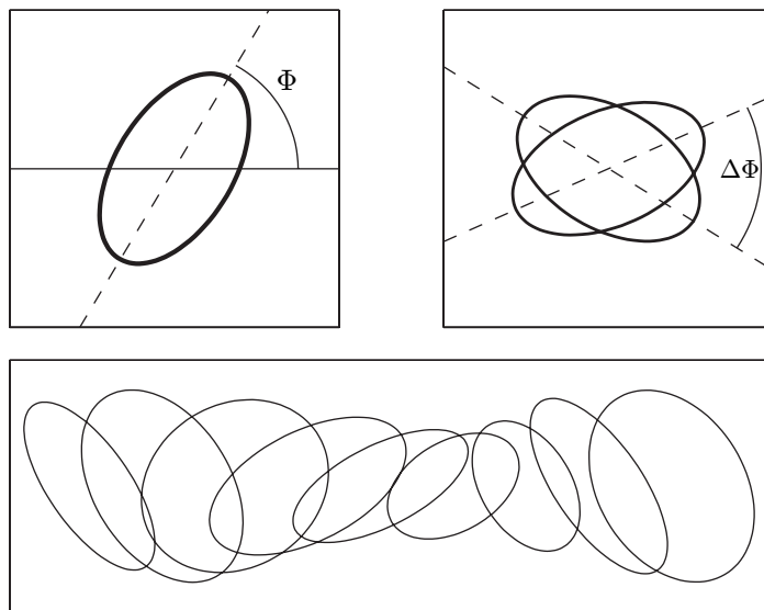
Figure 1. Vesicle projections to the shear plane in the tank-treading, trembling and tumbling regimes.
