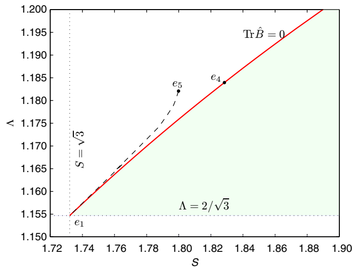
Figure 5. Phase diagram in the vicinity of the special point. Tank-treading to trembling transition.
