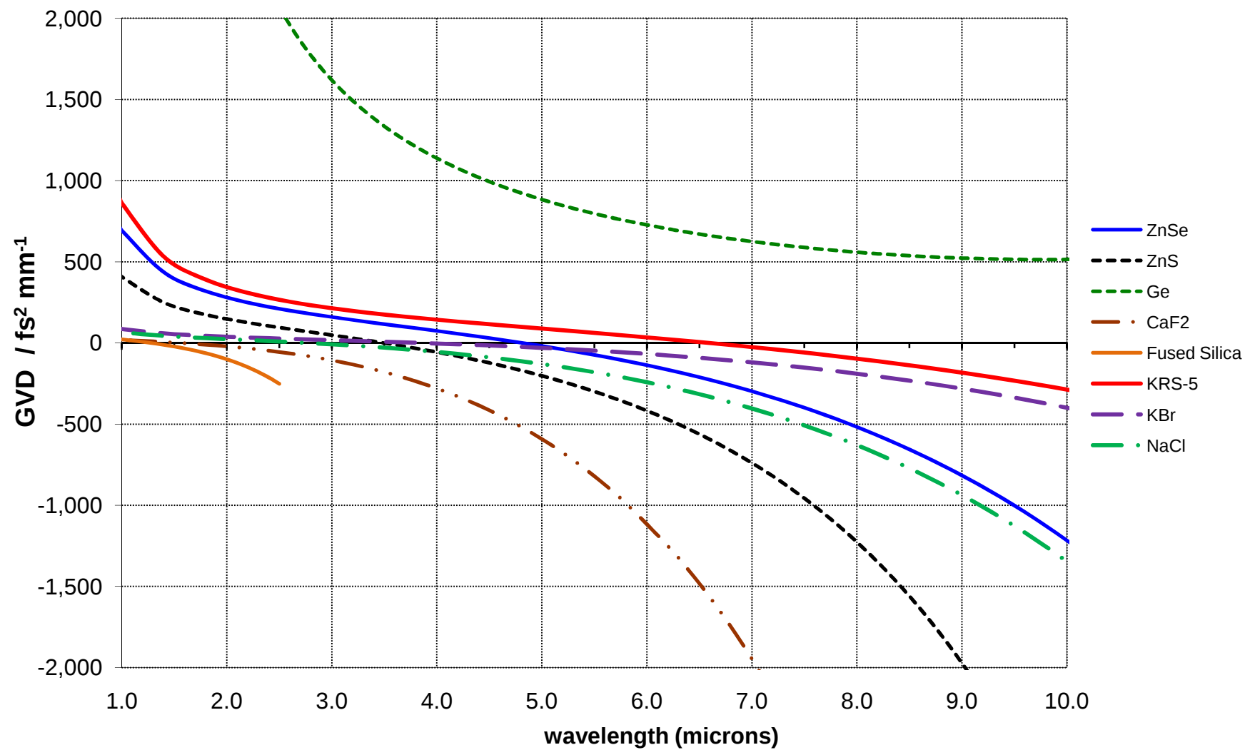
Group Velocity Dispersion (per mm of material)
