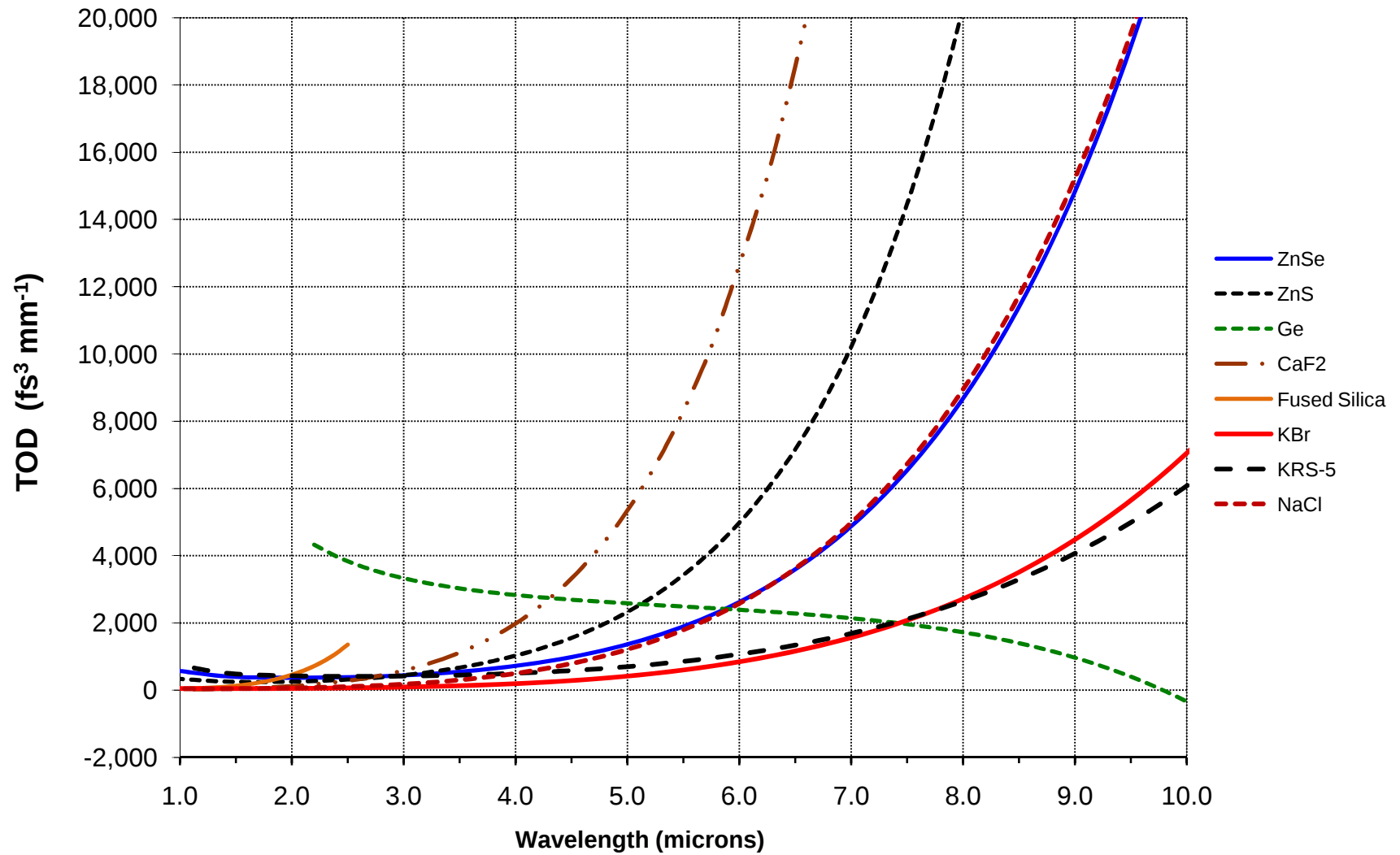
Third Order Dispersion (per mm of material)
