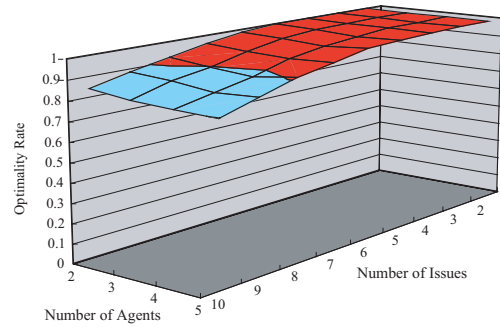
Figure 7: Scalability with the number of agents
