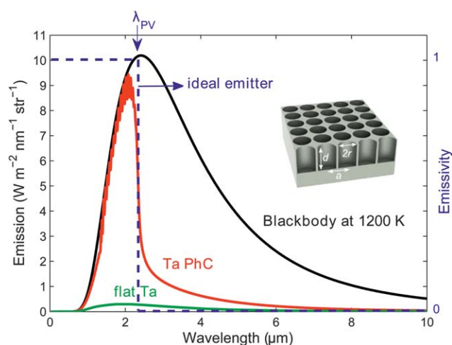
Fig. 1 (a) Simulated normal spectral emission at 1200 K of a Ta PhC optimized for a cutoff wavelength of \lambda = 2.3 \mu\text{m} (red) with radius r = 0.62 \mu\text{m} , a period a = 1.35 \mu\text{m} and an etch depth of d = 14.95 \mu\text{m} compared to that of flat Ta (green) and that of a blackbody emitter (black), and the emissivity of an ideal emitter (blue dashed line). Inset: schematic view of the PhC.
