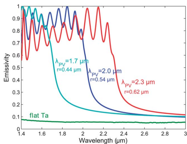
Fig. 2 Simulated normal emissivity of a Ta PhC optimized for a cut-off wavelength of \lambda = 2.3 \mu\text{m} (red), \lambda = 2.0 \mu\text{m} (blue) and \lambda = 1.7 \mu\text{m} (light blue) with the etch depth d restricted to 8 \mu\text{m} as compared to the emissivity of flat Ta (green).
