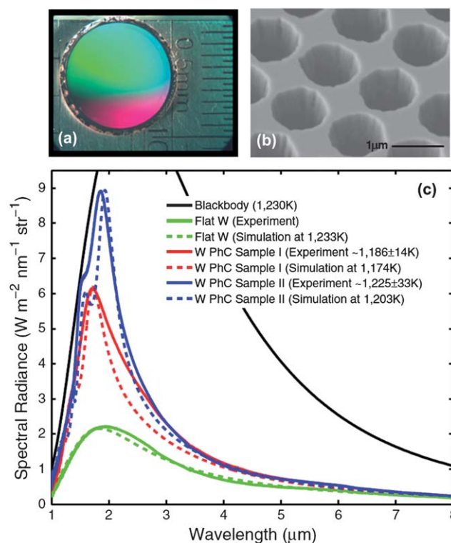
Fig. 4 Fabricated W PhC (Yeng et al. 25 ): (a) digital photo of the fabricated 1 cm diameter sample and (b) scanning electron micrograph of the fabricated W PhC. (c) Measured and simulated normal spectral emission obtained by heating the samples to ~1200 K as compared to emission from flat W (green) and ideal blackbody emission (black).
