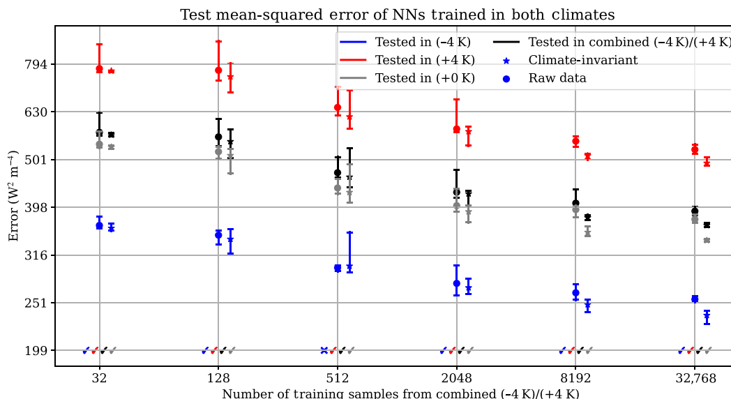
Fig. 8. Climate-invariant (CI) NNs trained on datasets containing both cold (-4 K) and warm (+4 K) samples outperform raw-data (RD) models offline in \approx 95\% of cases, with less sensitivity to the data partition used for training. Dots on the left represent the median RD error from a 10-fold cross-validation without replacement, with horizontal ticks indicating the first and ninth deciles. Stars on the right correspond to the median CI error. Ticks denote the majority of cases, for which CI models outperform RD models, even when data from both climates are available; crosses indicate the rare exceptions. We use a logarithmic scale for both axes.
