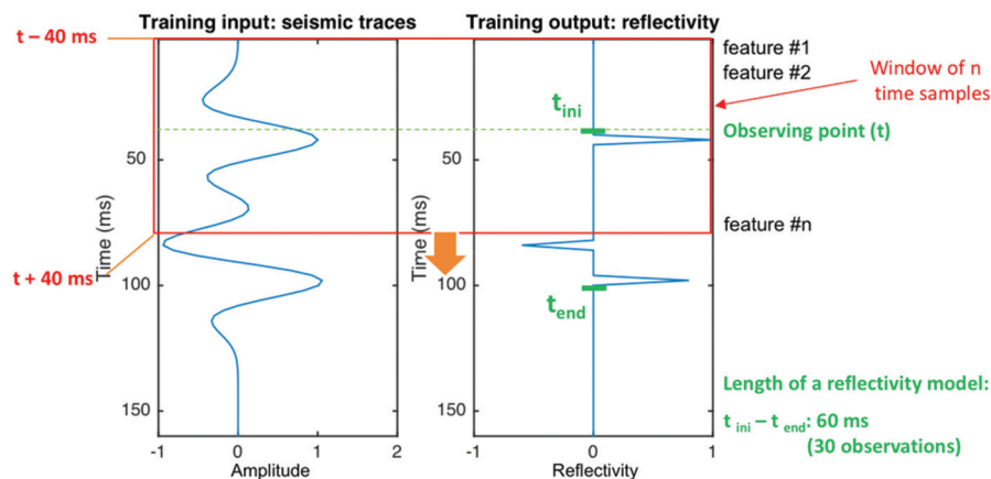
Figure 1. Description of training input and output data for reflectivity inversion using neural network methods.
