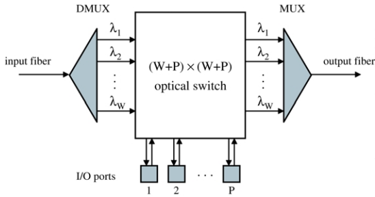
Fig. 1. An OADM architecture. Note that a (W + P) \times (W + P) switch is required, and that the size of this switch increases with the number of wavelengths.
