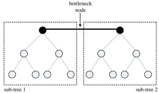
Fig. 12. A 14-node balanced binary tree. The bottleneck link is the link in heavy black; removal of this link from the graph disconnects the graph into the two indicated sub-trees, each containing |S_i^1| = |S_i^2| = 7 nodes. By considering all links in turn, it can be shown that this is the bottleneck link, resulting in a lower bound of seven wavelengths.
