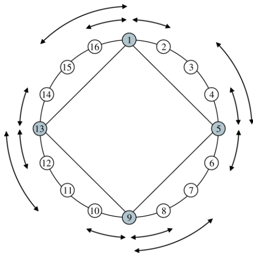
Fig. 5. Assigning local wavelengths for a single-port sixteen-node ring.
