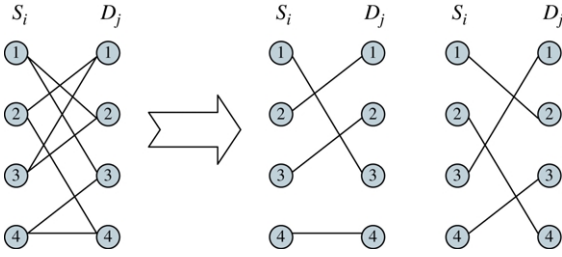
Fig. 9. The bridging graph for Example 2. As expected, each vertex in the bridging graph has vertex degree PC = 1 \cdot 2 = 2 . Using Theorem 1, this can be divided into C = 2 disjoint perfect matchings.
