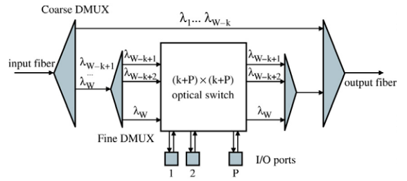
Fig. 2. An OADM architecture with bypass. Note that the switch size depends only on the number of wavelengths k entering the node, not the total number W .
