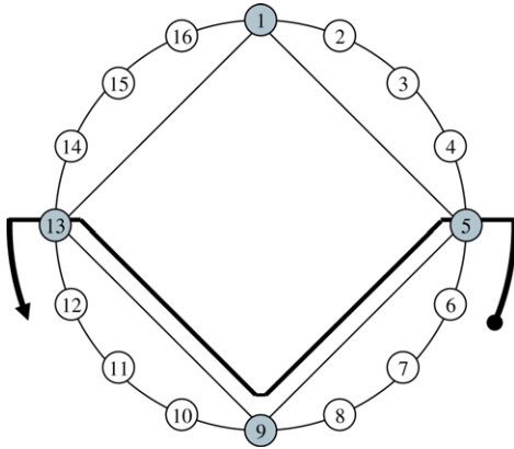
Fig. 6. The route for call (6, 12). Hubs 5 and 13 are used to access the bypass wavelengths.
