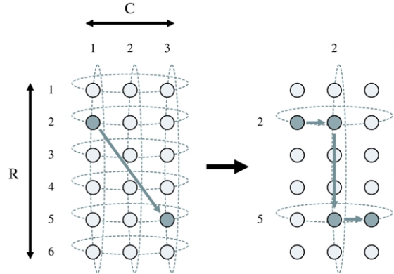
Fig. 7. Breaking up a call into three sub-calls using a bridging column. The single call on the left, from n_{2,1} to n_{5,3} , is routed as two row-ring calls and a column-ring call using the bridging column 2. Each of the sub-calls can be routed independently on their respective rings using the \lceil PN/4 \rceil algorithm. Additional wavelength conversion may be required at nodes n_{2,2} and n_{5,2} if the sub-calls are not assigned to the same wavelength.
