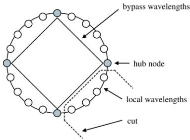
Fig. 4. A dual ring topology, equivalent to a twenty-node, four-hub ring with some local and some bypass wavelengths. The shaded nodes are hubs.
