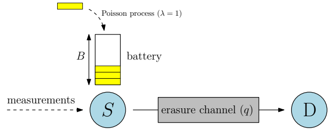
Fig. 7. System model for status updating over erasure channels. Updates packets are erased with probability q . The channel is noiseless when q = 0 .
