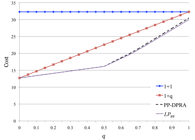
Fig. 5: Cost vs. q for various protection schemes
