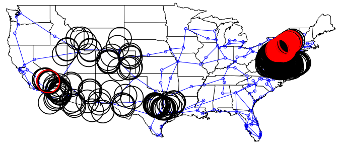
Fig. 11. The impact of circular cuts of radius 2 on the MFST between Los Angeles and NYC. Red circles represent cuts that result in MFST = 0 and black circles result in MFST = 1 . Cuts which intersect the nodes representing Los Angeles or NYC are not shown.
