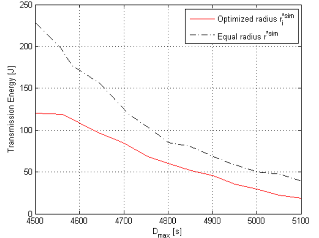
Fig. 5. Transmission energy versus the maximum delay D_{max} both for optimized radii r_i^{*sim} and equal radii r_i^{*sim} .
