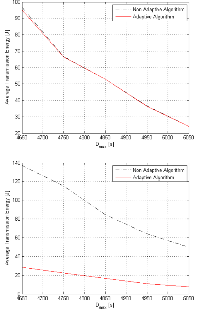
Fig. 7. Average transmission energy versus the delay constraint D_{max} for the Poisson arrival case (top) and for the Bernoulli case (bottom), considering both the stochastic algorithms.
