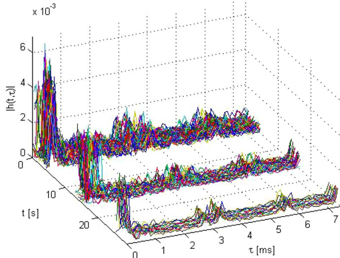
Fig. 16. Estimated channel impulse responses (magnitude) for packets 1-3; element 1 in the low-speed case.
