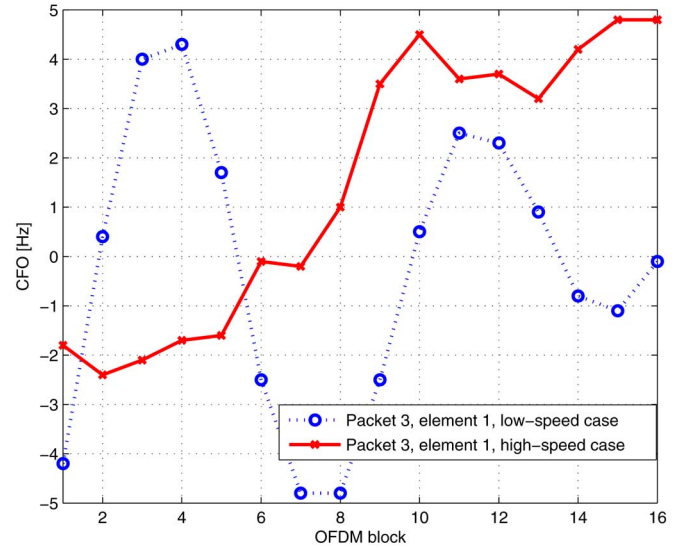
Fig. 15. Estimated residual Doppler of packet 3. K = 2048 and each packet has 16 OFDM blocks.
