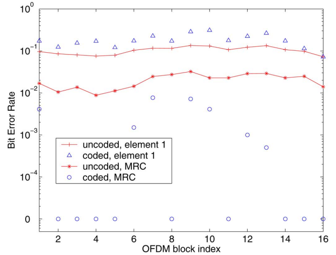
Fig. 18. BERs for each OFDM block, the low-speed case, K = 2048 .
