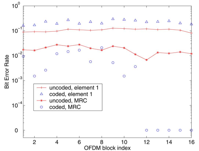
Fig. 19. BERs for each OFDM block, the high-speed case, K = 2048 .
