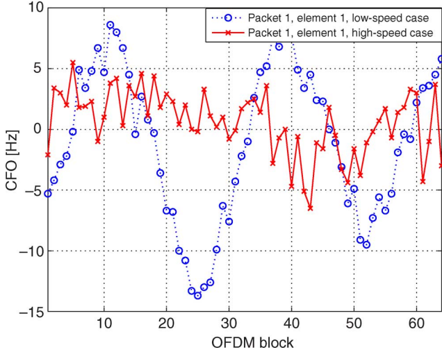
Fig. 13. Estimated residual Doppler shift of packet 1. K = 512 and each packet has 64 OFDM blocks.
