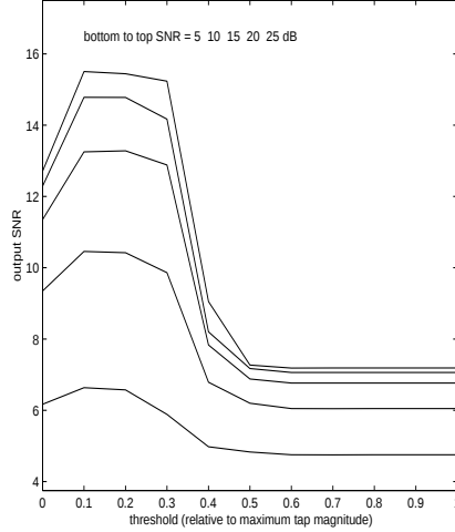
Fig. 3. SNR at the equalizer output as a function of the threshold used for sparsifying the channel estimate. The input SNR is determined by the AWGN power. Threshold is given relative to the absolute value of the maximum channel coefficient: a threshold of 0 indicates that all coefficients are kept in the channel estimate used for post-cursor ISI calculation, while a threshold of 1 indicates that only one (the strongest, or the reference coefficient) is kept. The feedforward equalizer uses 3 contiguously spaced taps around the reference tap; the channel estimate has 19 coefficients. The curves are obtained by averaging 500 independent simulation runs.
