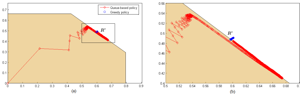
Fig. 8. Average allocated rates by greedy and queue-length based policies approaching the optimal solution \mathbf{R}^* of maximizing the utility function over the average capacity region. Part (b) is a magnification of the box in part (a) to demonstrate behavior of the policies in the neighborhood of the optimal solution. The queue-based policy approaches \mathbf{R}^* from the interior of the region, while the greedy policy approaches \mathbf{R}^* from the exterior.
