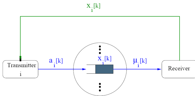
Fig. 5. Structure of the i -th transmitter and the receiver for the queue-length-based policy [8].
