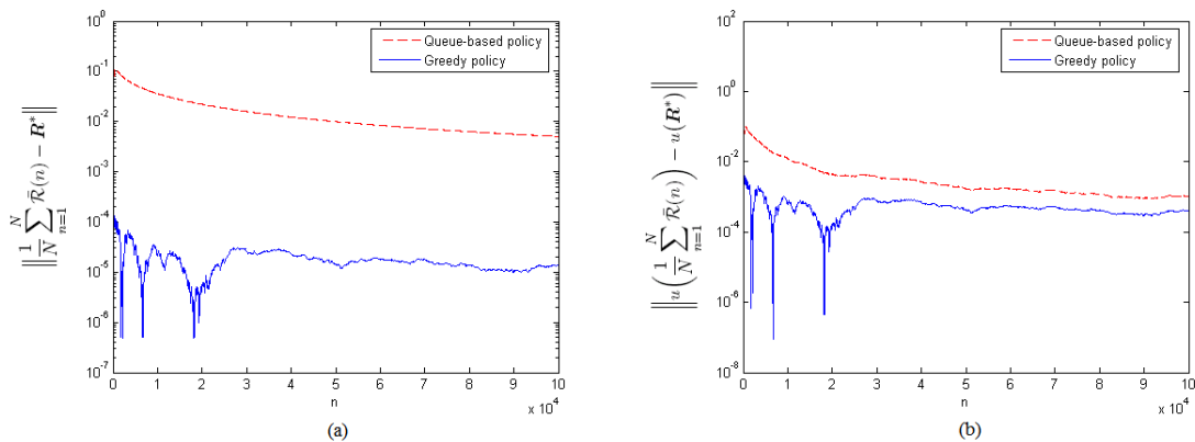
Fig. 7. Performance comparison of greedy and queue-based policies for a communication session with limited duration, for \sigma_H = 0.13 .
