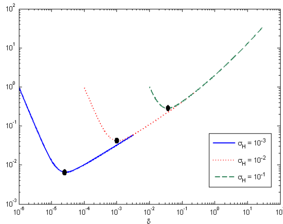
Fig. 3. Parametric upper bound on performance difference between greedy and long-term optimal policies as in right hand side of (43) for different channel variations, \sigma_H , as a function of \delta
