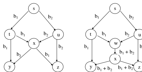
Figure 1 Networks with multicast connection from s to y and z .
