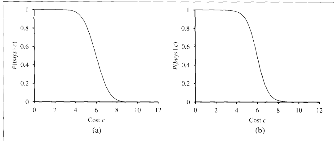
Figure 14.7 (a) A probit distribution for the probability of Buys given Cost , with \mu = 6.0 and \sigma = 1.0 . (b) A logit distribution with the same parameters.
