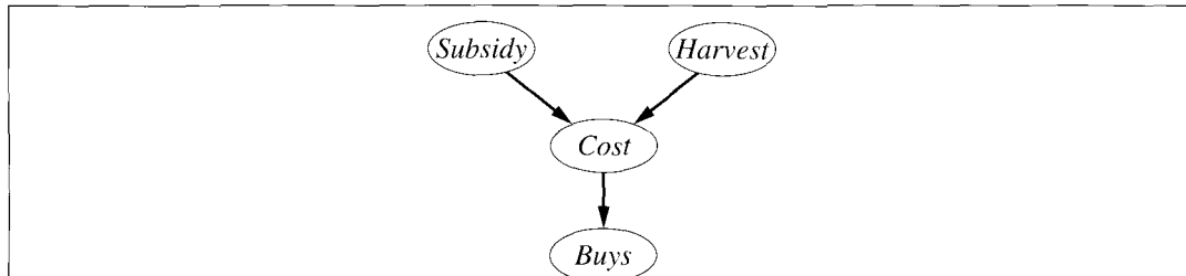
Figure 14.5 A simple network with discrete variables ( Subsidy and Buys ) and continuous variables ( Harvest and Cost ).
