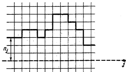
FIG. 1. Schematic diagram of a step on the basal plane of a crystal with a simple cubic lattice (view from above). In the SOS approximation it is assumed that the configuration of the step can be specified by a set of integer variables n_j which give the distance of the step from some fixed position.
