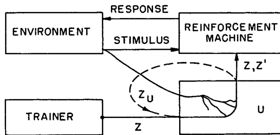
Fig. 9—An additional device U gives the machine of Fig. 8 the ability to learn which signals from the environment have been associated with reinforcement. The primary reinforcement signals Z are routed through U . By a Pavlovian conditioning process (not described here), external signals come to produce reinforcement signals like those that have frequently succeeded them in the past. Such signals might be abstract, e.g., verbal encouragement. If the "secondary reinforcement" signals are allowed, in turn, to acquire further external associations (through, e.g., a channel Z_U as shown) the machine might come to be able to handle chains of subproblems. But something must be done to stabilize the system against the positive symbolic feedback loop formed by the path Z_U . The profound difficulty presented by this stabilization problem may be reflected in the fact that, in lower animals, it is very difficult to demonstrate such chaining effects.
