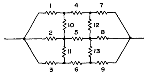
Fig. 11—This board game (due to C. E. Shannon) is played on a network of equal resistors. The first player's goal is to open the circuit between the endpoints; the second player's goal is to short the circuit. A move consists of opening or shorting a resistor. If the first player begins by opening resistor 1, the second player might counter by shorting resistor 4, following the strategy described in the text. The remaining move pairs (if both players use that strategy) would be (5, 8) (9, 13) (6, 3) (12, 10 or 2) (2 or 10 win). In this game the first player should be able to force a win, and the maximum-current strategy seems always to do so, even on larger networks.
