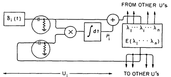
Fig. 1—"Multiple simultaneous optimizers" search for a (local) maximum value of some function E(\lambda_1, \dots, \lambda_n) of several parameters. Each unit U_i independently "jitters" its parameter \lambda_i , perhaps randomly, by adding a variation \delta_i(t) to a current mean value \mu_i . The changes in the quantities \delta_i and E are correlated, and the result is used to (slowly) change \mu_i . The filters are to remove dc components. This simultaneous technique, really a form of coherent detection, usually has an advantage over methods dealing separately and sequentially with each parameter. (Cf. the discussion of "informative feedback" in Wiener [11], p. 133 ff.)
