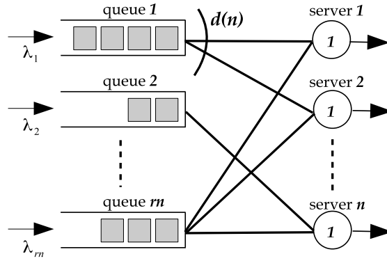
Figure 2 A processing network with n queues and n servers.
