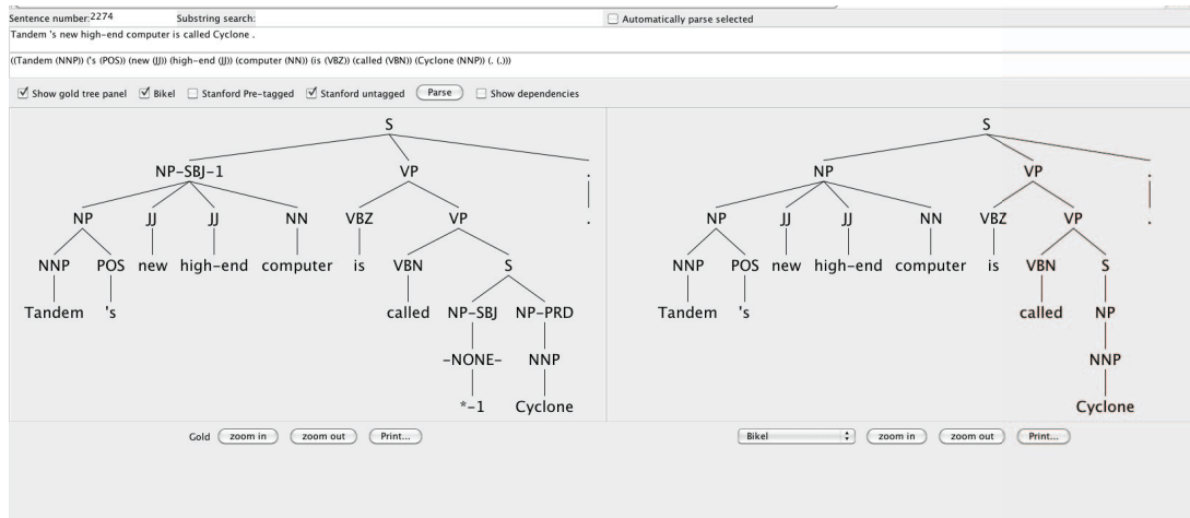
Figure 6. The Bikel/Collins parser analysis of sentence #2274 of section 23 of the PTB. The gold standard annotation is on the left, the parser output on the right.
