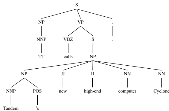
Figure 7. The parse of regularized sentence #2274 mis-analyzes the NP – NP structure under a single NP, precision=71.433%, recall=83.333%.
