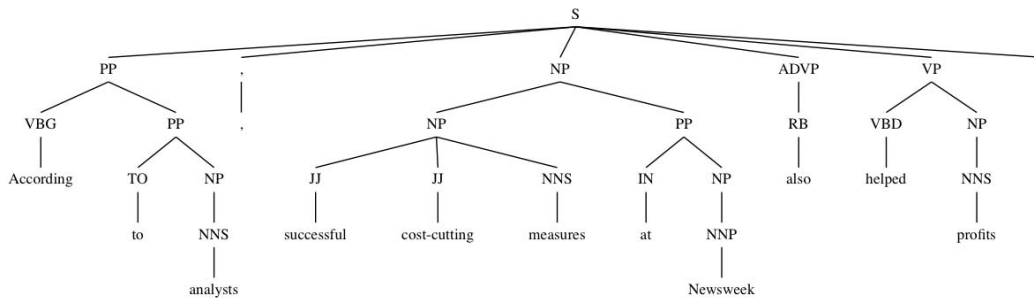
Figure 5. The Bikel/Collins parser mis-analyzes of sentence # 722 in section 23 of the PTB. The top half of the figure shows the result of parsing the original sentence. The bottom half shows the result of parsing the same sentence correctly after the regularization procedure described in the main text.
