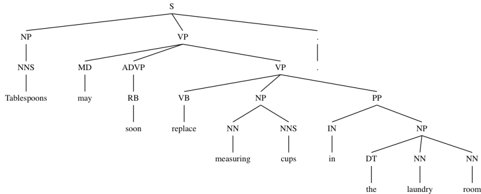
Figure 4. The Bikel/Collins parser correctly analyzes the “tablespoon” sentence after regularization.
