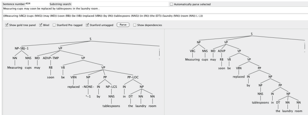
Figure 1. Stanford and Bikel/Collins mis-parses of sentence number 404 in the PTB. The left-hand panel shows the correct, “gold standard” structure. The right-hand panel displays the result of parsing the same sentence using Bikel’s reimplementation of the Collins parser and the Stanford parser, which produce the same erroneous parse.
