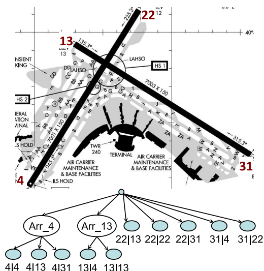
Fig. 2. Layout of LGA, along with the estimated NL structure for LGA configuration selection (for year 2006).
