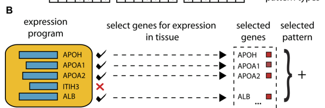
Figure 3. Overview of the GeneProgram Probability Model, Which Is Based on Hierarchical Dirichlet Process Mixture Models
