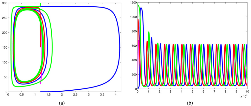
Fig. 7. (a) Projections of solutions into \lambda, z_3 plane and (b) the y_3 as a function of time, for four different initial conditions. The matching colors in these two figures correspond to the same initial condition. See footnote 3.
