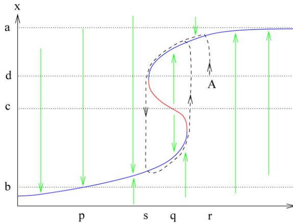
Fig. 1. Relaxation from bistability.
