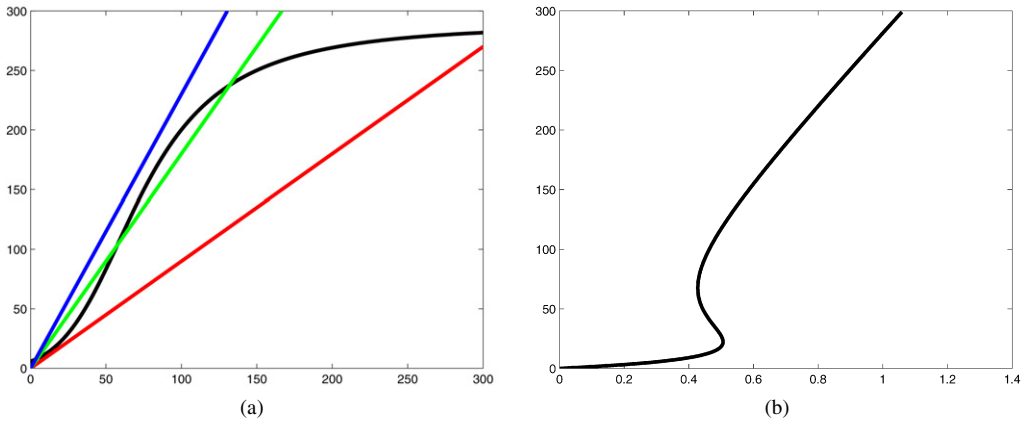
Fig. 6. (a) The graph of the function k(u) and lines with slopes 0.9, 1.8 and 2.3. (b) The set of equilibria of the system (5) as a function of \lambda . These are the intersections of the graph of k(u) and the lines \frac{1}{\lambda}u .
