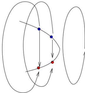
Fig. 3. Limit point bifurcation gives rise to a stable periodic orbit.
