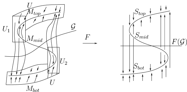
Fig. 4. Map F maps the 2-dimensional manifold in the neighborhood of the set M to its image in \mathbf{R}^2 . The flow \psi (left figure), generated by (4), is orbit equivalent to the flow \varphi (right figure), generated by (13). The neighborhoods U_1 and U_2 of the turning points on M are also indicated.
