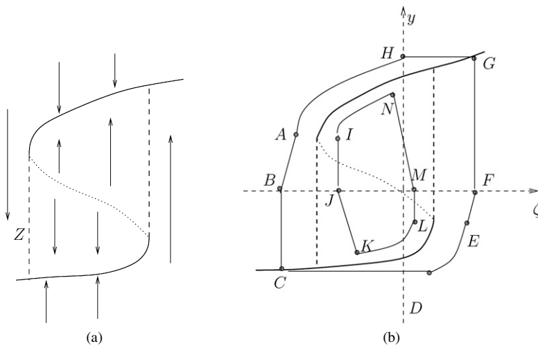
Fig. 2. (a) The Z curve, (b) the set N in the neighborhood of the Z curve, that is positively invariant under the flow of (12).
