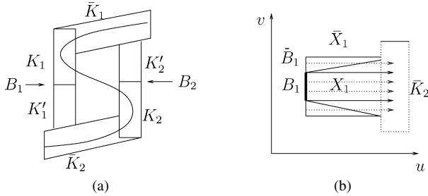
Fig. 5. (a) A projection of various sets into 2-dimensional manifold \tilde{U} . (b) Shaving between flow boxes X and \bar{X} . The picture on the right is in complementary directions to the picture on the left.
