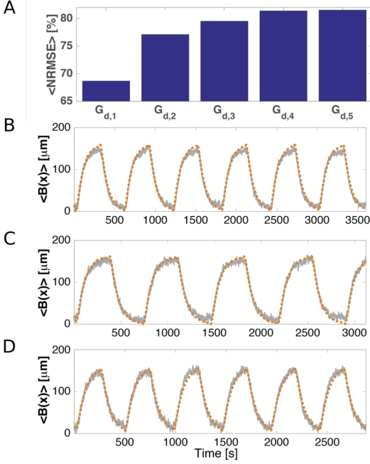
Fig. 2. System Identification results. (A) Summary of the \langle NRMSE \rangle for the models in Table 1. (B)-(D) Experimentally measured center of mass \langle B(x) \rangle , in gray, for three of the 10 experiments in our dataset, plotted with the prediction, dashed orange line, from the selected model, G_{d,4} .
