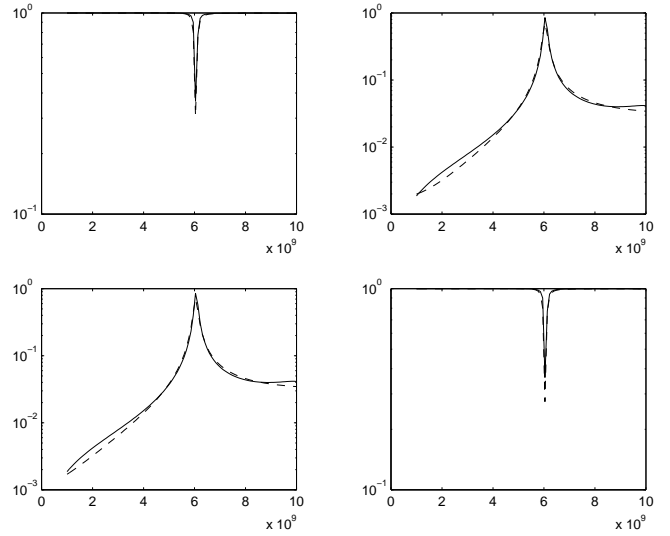
Figure 2: Magnitude of rational function fit and reduced model for S-parameters tabulated by full-wave field solver. Solid line shows initial data and order-42 rational fit (complete overlap). Dashed line shows order-6 reduced model obtained via BR-TBR.
