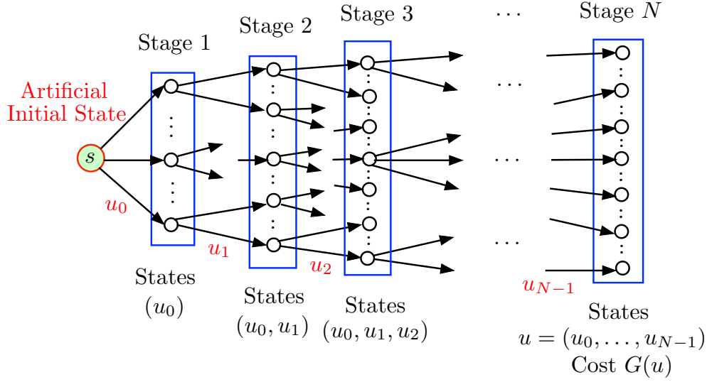
Figure 3.1. Formulation of a discrete optimization problem as a DP problem with N stages. Starting with an artificial initial state, a new control component is chosen at each stage. There is a cost G(u) only at the terminal stage.
