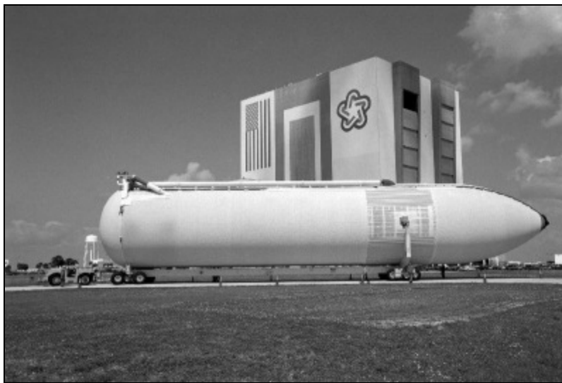
Figure 15 – Space shuttle external fuel tank 15
