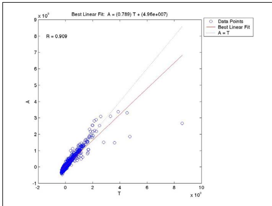
Figure 12 – Structures model neural network performance predicting cone stress (R~0.91)
