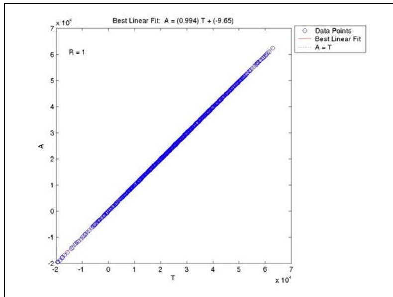
Figure 38 – Aerodynamics model neural network performance predicting payload ( R \sim 1 )
