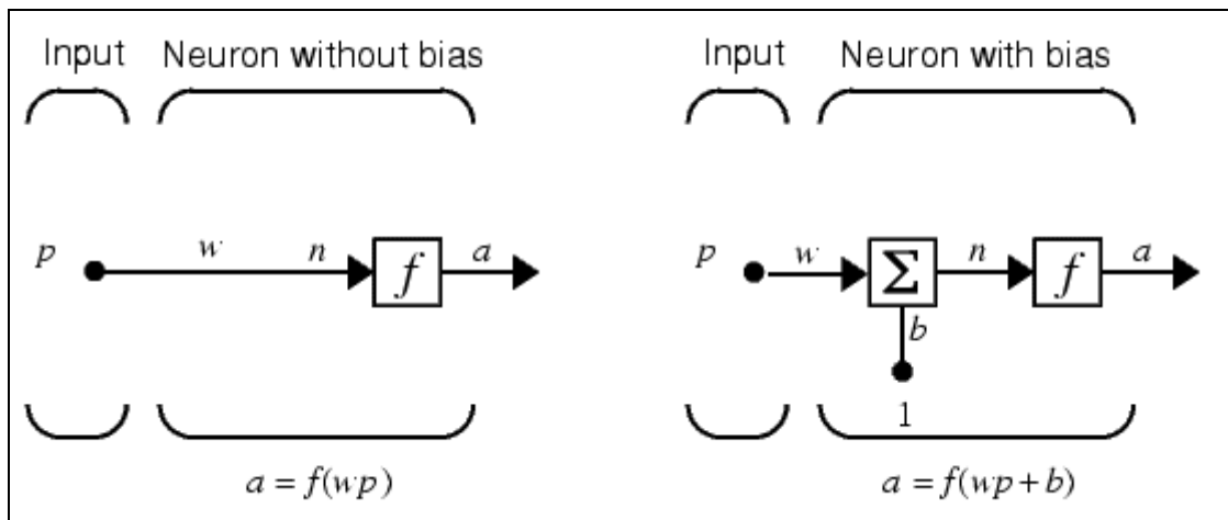
Figure 5 – Simple Neuron Model 10
