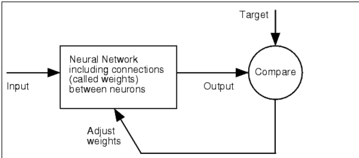
Figure 4 – Neural network iteration loop 10
