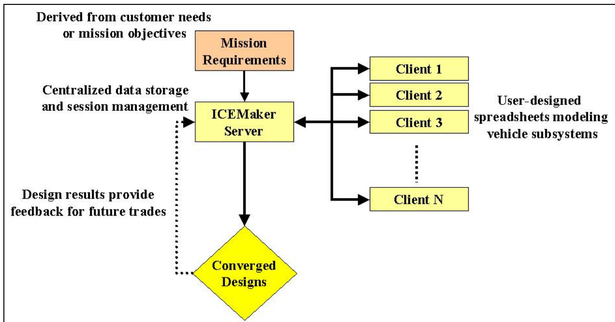
Figure 1 – ICEMaker setup
