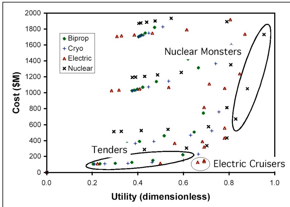
Figure 36 – Promising designs
