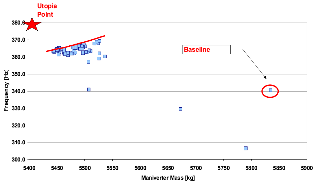
Fig. 124: Testing Phase – Frequency-Mass Trade-Space
