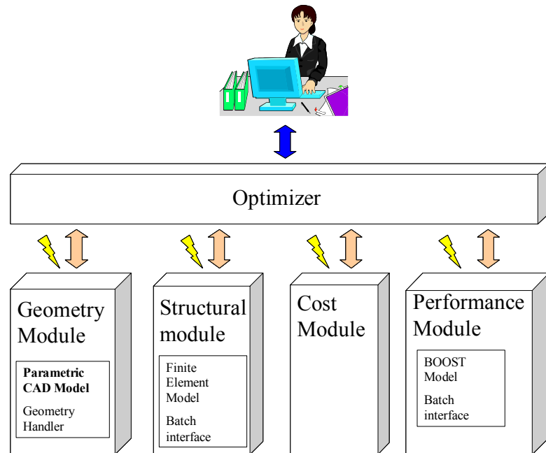
Fig. 58: Overview of the ICE platform Architecture:
