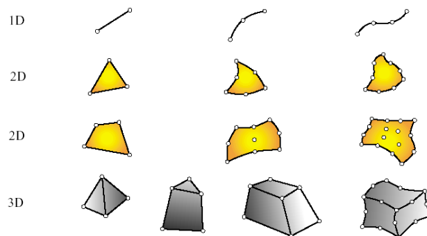
Fig. 74: Finite Element Types
