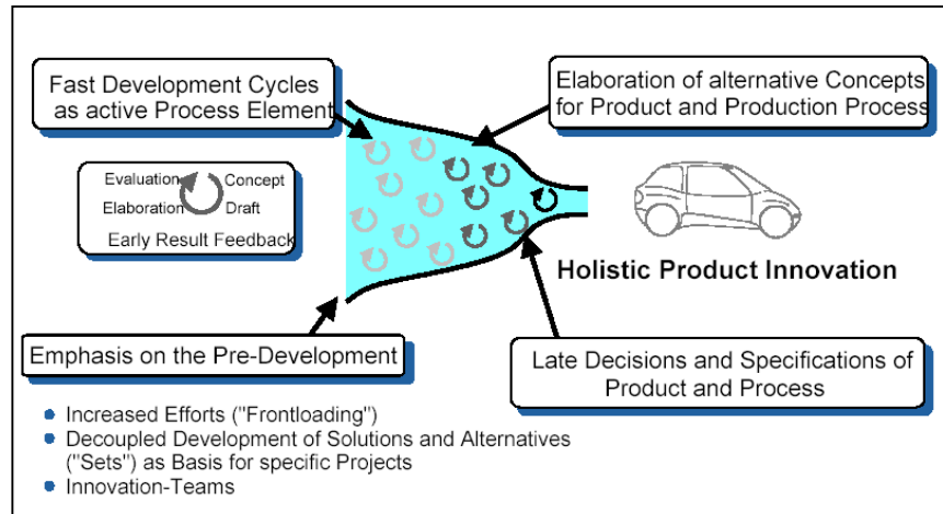
Fig. 21: Evolutionary-Iterative Development
