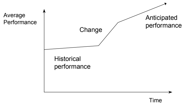
Fig. 141: Change: common expectations
