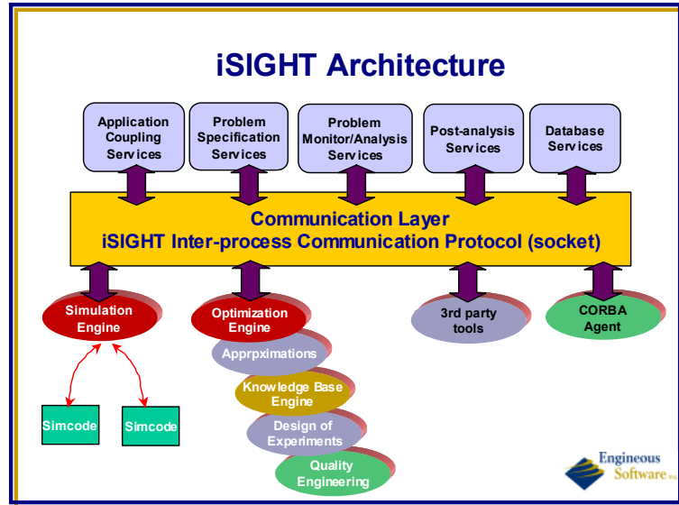
Fig. 94: iSIGHT Architecture
