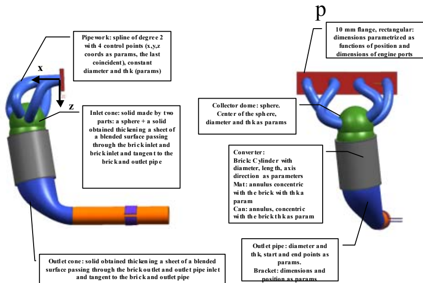
Fig. 19: The Full Maniverter
