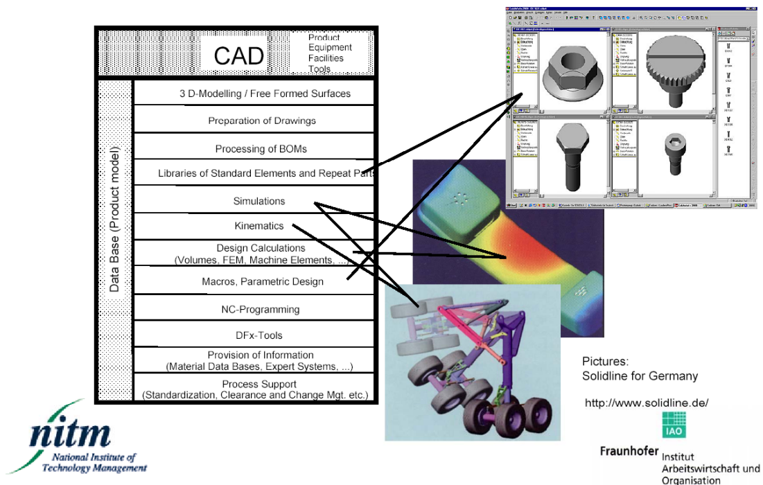
Fig. 61: CAD Functionalities
