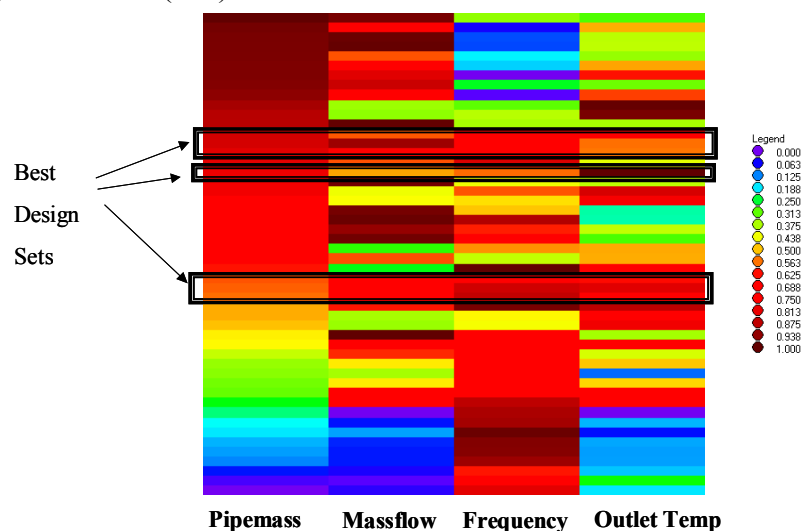
Fig. 109: Qualitative Rainbow Plot of Simple Pipe Pareto Designs
