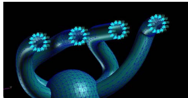
Fig. 81: Boundary Conditions applied to the Pipework
