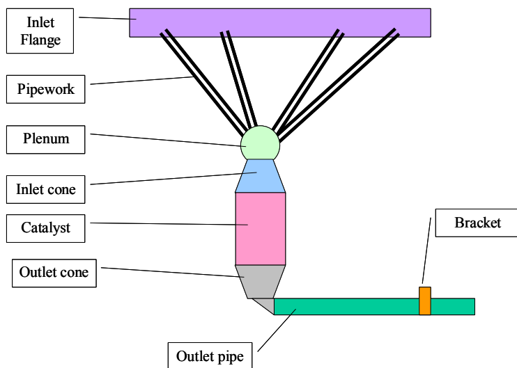
Fig. 64: Simplified Maniverter Concept
