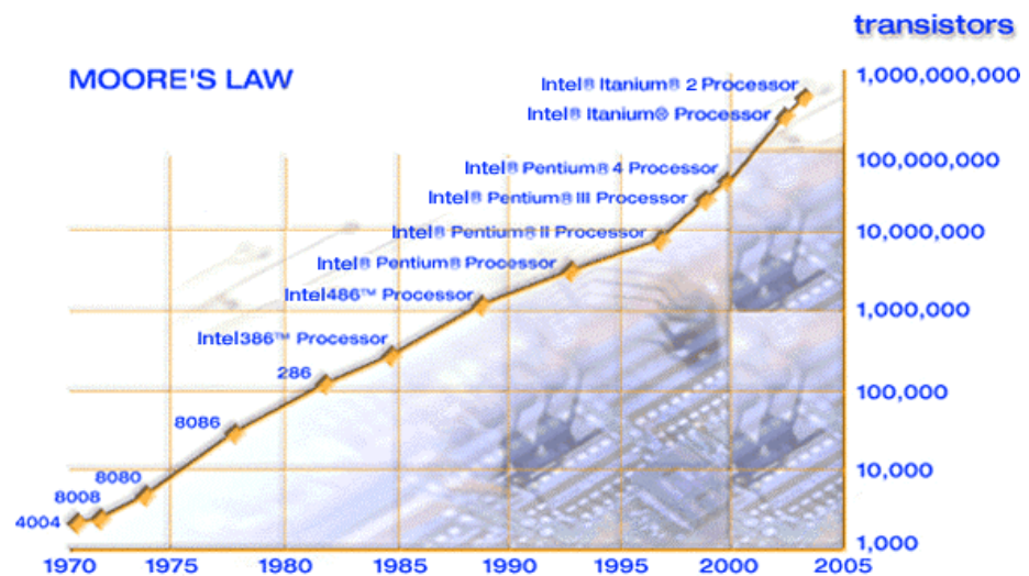
Fig. 30: Moore's Law
