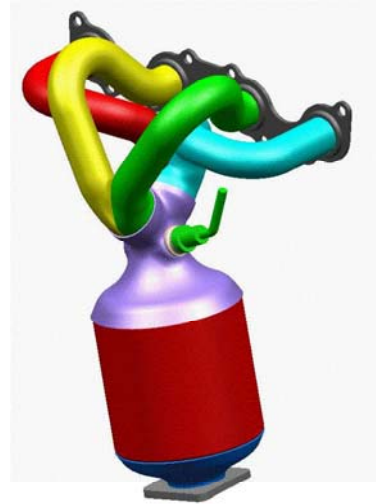
Fig. 56: An Example of a Maniverter
