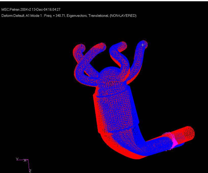
Fig. 84: Modal Shape Visualization (global lateral mode)
