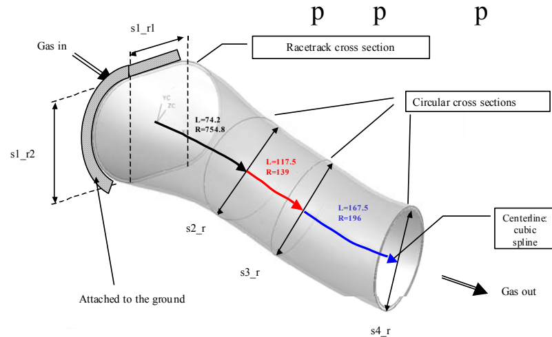
Fig. 18: The Simple Pipe
