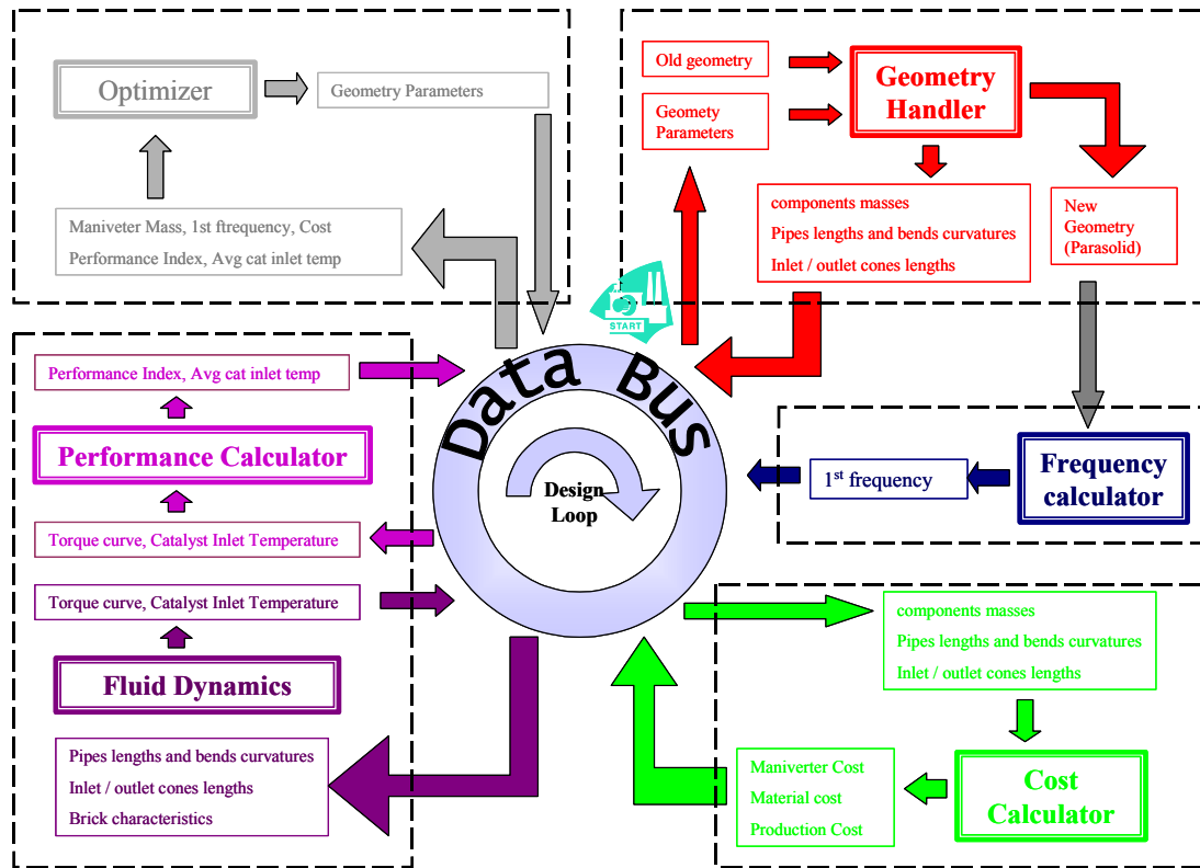
Fig. 97: ICE Platform Data Flow
