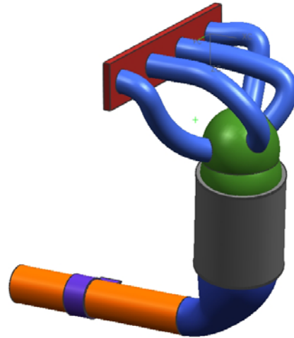
Fig. 123: Testing Phase – Cost Minimization – Resulting Geometry
