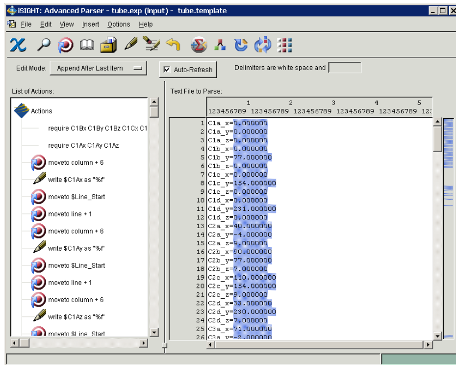
Fig. 99: Input File Parsing Sample
