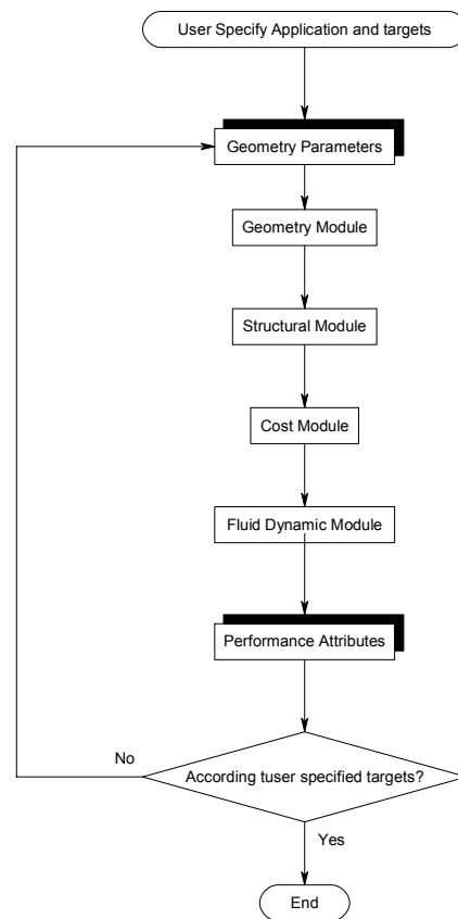
Fig. 59: Flowchart of the design loop execution
