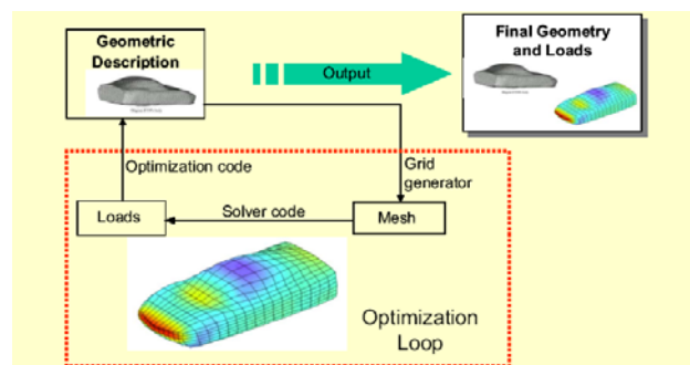
Fig. 42: Scheme of the aerodynamic optimization procedure
