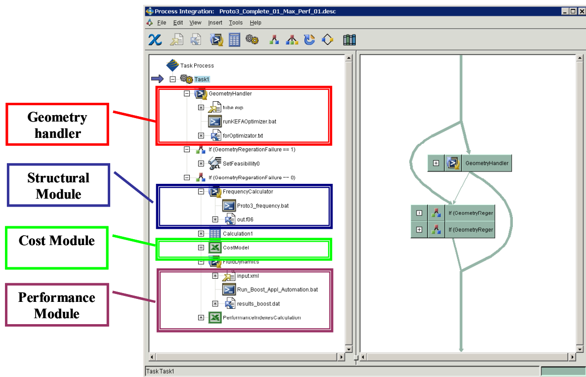
Fig. 96: The iSIGHT Implementation of the ICE Platform
