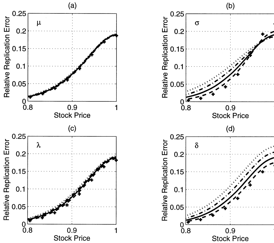
Figure 12. The relative replication error of a 6-month maturity European option to “sell at the high” (relative to the replication cost), plotted as a function of the initial stock price. The stock price follows the mixed jump-diffusion process (3.20)–(3.23), (3.26), (4.1), and (4.2) with parameter values m = 1 , \mu = 0.07 , \sigma = 0.106 , \lambda = 25 , and \delta = 0.015 corresponding to the solid line. In Panels (a)–(d), \mu , \sigma , \lambda , and \delta are each varied, respectively, while the other parameter values are held fixed. The variation in each parameter is obtained by multiplying its original value by 1.25 (dashed-dotted line), 1.5 (dots), 0.75 (dashed line), and 0.5 (pluses).
