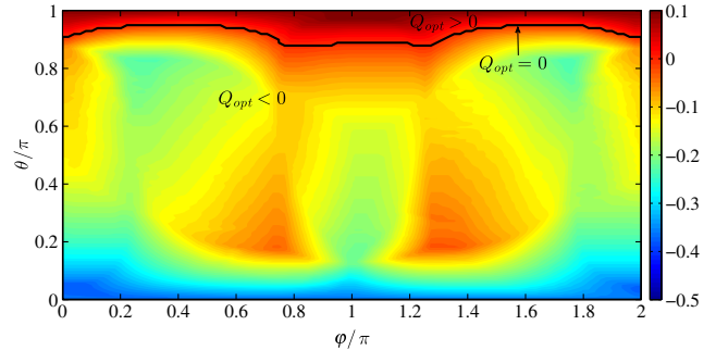
a) Aircraft optimum charge, in mC
