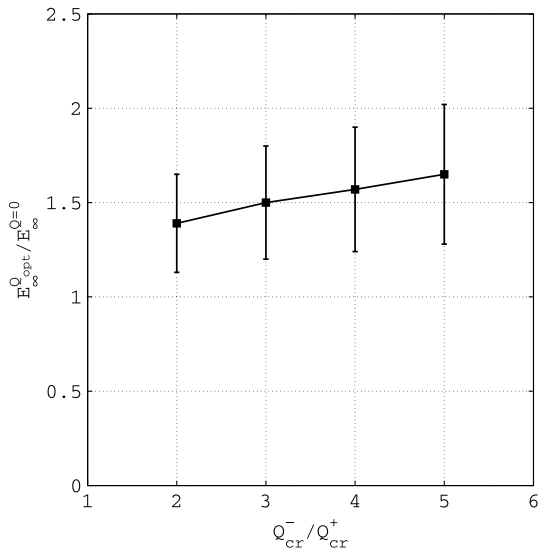
Fig. 7 Gain of the charge control strategy E_{\infty}^{0_{opt}} / E_{\infty}^{0=0} as a function of the degree of asymmetry Q_{cr}^- / Q_{cr}^+ . Equiprobability of ambient field orientation has been assumed. Critical positive corona charge is kept at Q_{cr}^+ = 1 \mu C .
