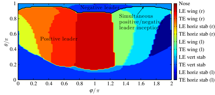
a) Baseline case, Q_{ac} = 0 : first attachment
