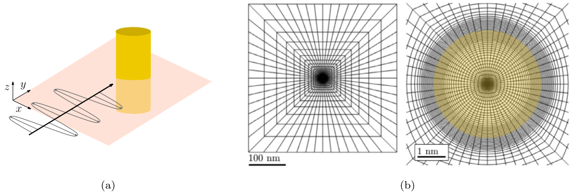
Fig. 2. (a) Schematic diagram of single nanowire under plane wave illumination. (b) Two views of the cubic discretization, with gold nanowire highlighted.
