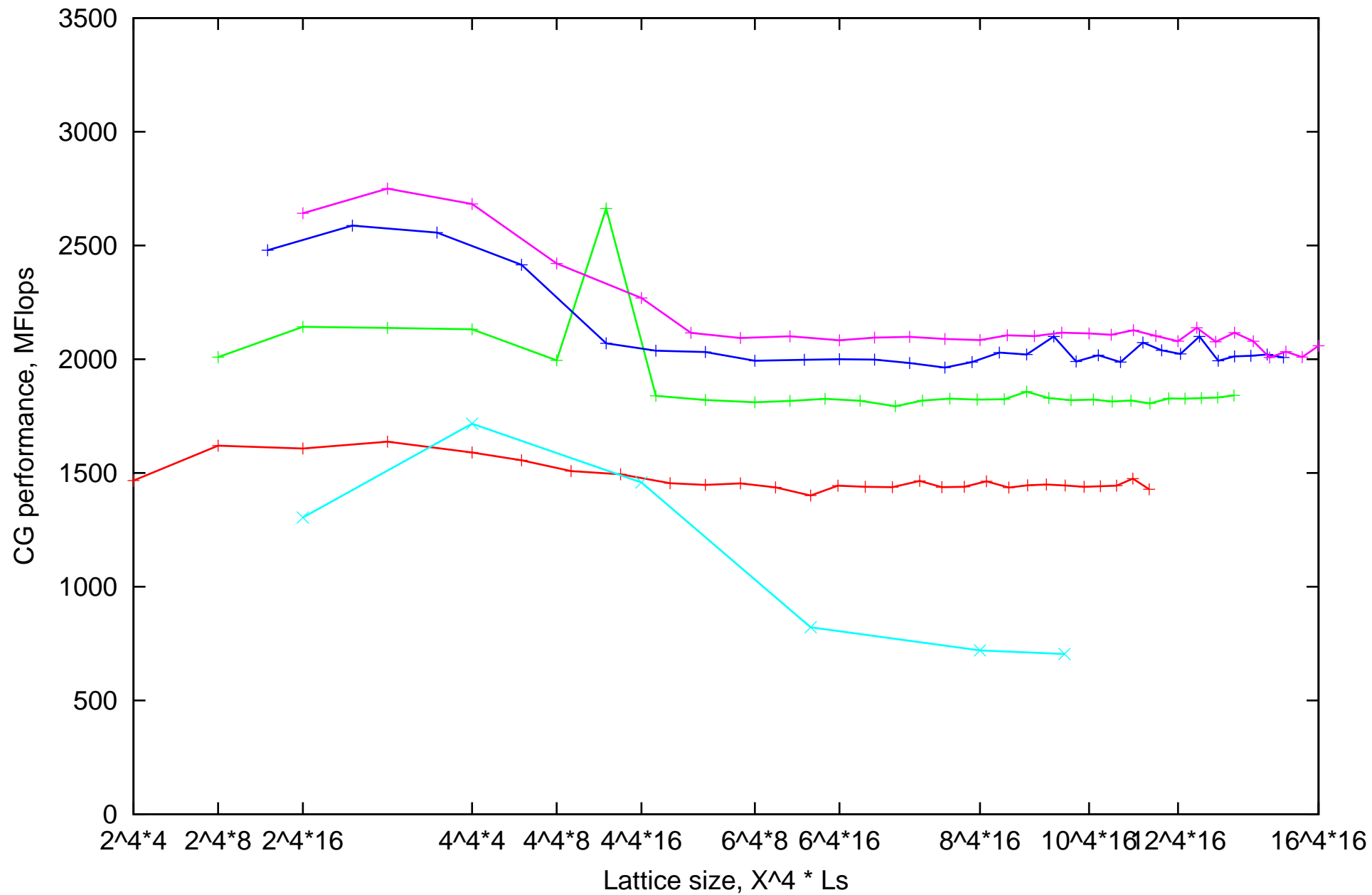
Single node performance of DWF CG on 2.66GHz Xeon (JLab qcd3g cluster)
