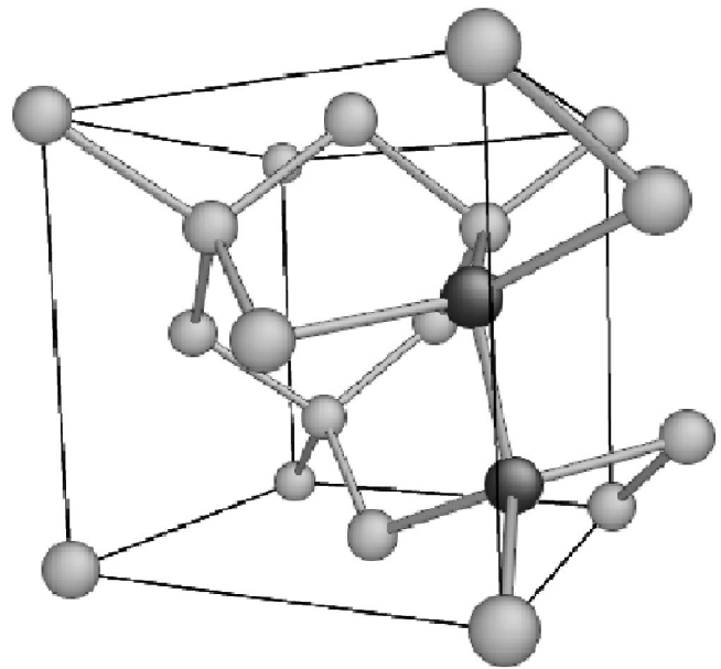
FIG. 6. The fourfold coordinated defect referred to a unit cell. The two displaced atoms are darkened.
