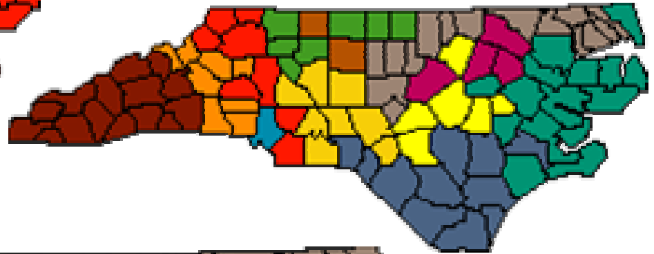
Greedy algorithm
