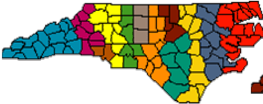
Cake-cutting algorithm
