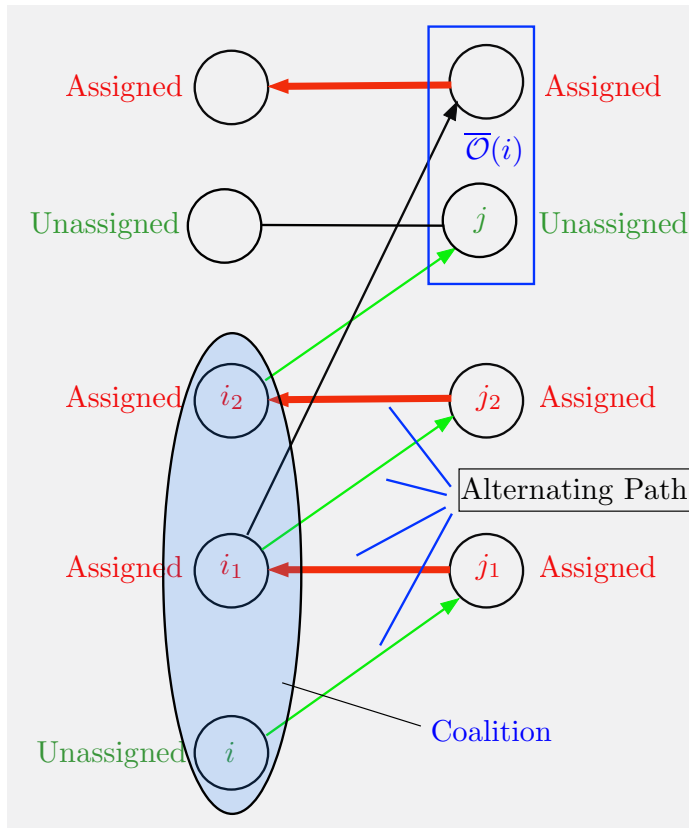
Figure 3.12 Illustration of the cooperative auction iteration, where after raising the prices, there is an object in the set \bar{O}(i) that is unassigned. Then, we may optionally perform an augmentation, shown in green, along a corresponding augmenting path [(i, i_1, i_2, j)] in the figure]. In particular, persons i , i_1 , and i_2 get assigned to j_1 , j_2 , and j , respectively.
