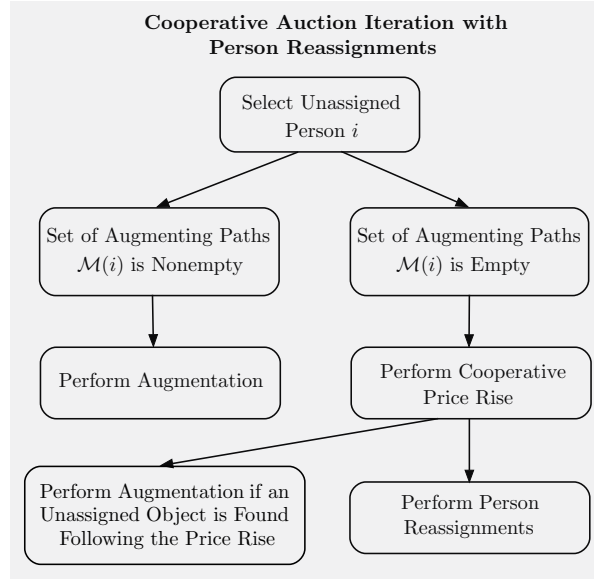
Figure 4.2 Block diagram of a cooperative auction iteration with person reassignments. Here, if an unassigned object is not discovered following a cooperative price rise, person i assigned through a reassignment of the coalition persons and a rearrangement of the corresponding assigned pairs.
