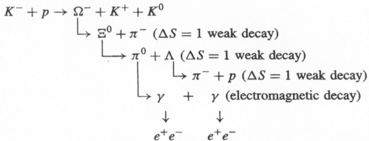
Fig. 4.11. The first \Omega^- event (Barnes et al. 1964), courtesy Brookhaven National Laboratory). It depicts the following chain of events:
