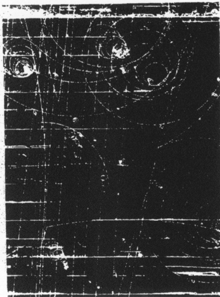
Fig. 4.11. The first \Omega^- event (Barnes et al. 1964), courtesy Brookhaven National Laboratory). It depicts the following chain of events:
