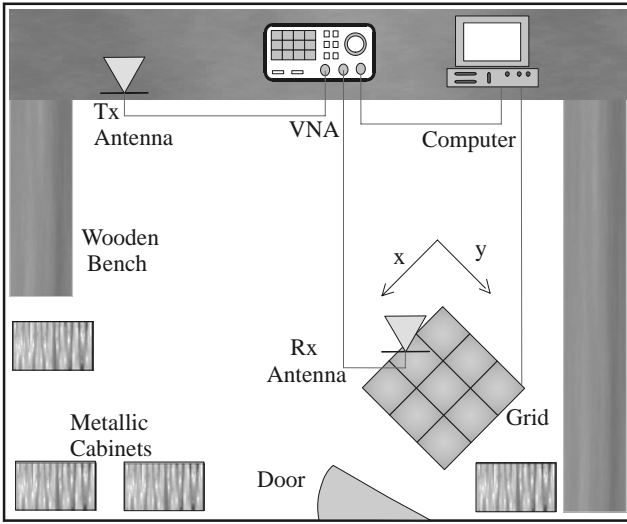
Fig. 1. Indoor MIMO channel measurement system
