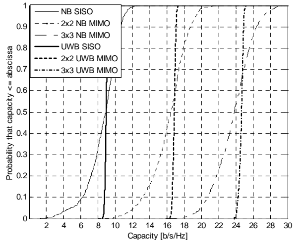
Fig.8. Spectral efficiency (NLOS)
