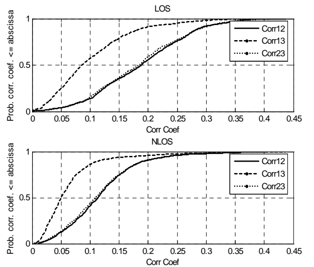
Fig. 3. Cumulative distribution function of receive correlation
