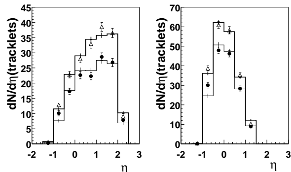
FIG. 3. Tracklet pseudorapidity density in the detector acceptance per event for data at \sqrt{s} = 56 (circles) and 130 AGeV (triangles) for SPEC (left) and VTX (right), in comparison to scaled HIJING simulations (solid lines).
