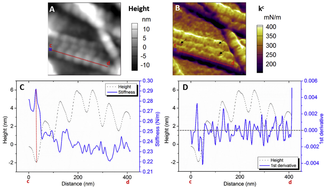
Fig. 5. Dual-frequency AFM images of oim/oim collagen fibers ( 0.5 \times 0.5 \mu\text{m}^2 , 256 \times 256 pixels). (A) Topography. (B) Stiffness mapping. (C) Stiffness data profile along the line c-d with corresponding topography profile. (D) First derivative of stiffness profile indicates the locations of stiffness changes along the fiber. The results showed the organized periodic pattern of oim/oim collagen fiber, but no correlation to the stiffness distribution. The stiffness fluctuates randomly along the fiber, without any recognized repeated pattern.
