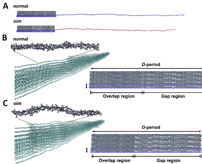
Fig. 3. Molecular modeling of +/+ and oim/oim collagen molecules. (A) Molecular structures. The blue box shows the triclinic unit cell of the full atomistic +/+ and oim/oim fibrils. (B) and (C) shows the structural differences between +/+ and oim/oim collagen at single molecular and fibril levels respectively. (For interpretation of the references to colour in this figure legend, the reader is referred to the web version of this article.)
