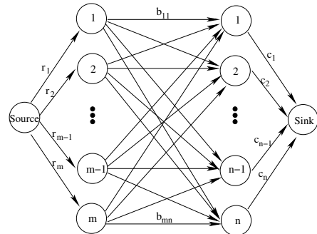
Fig. 1. Equivalence of feasibility problem to maximum-flow problem
