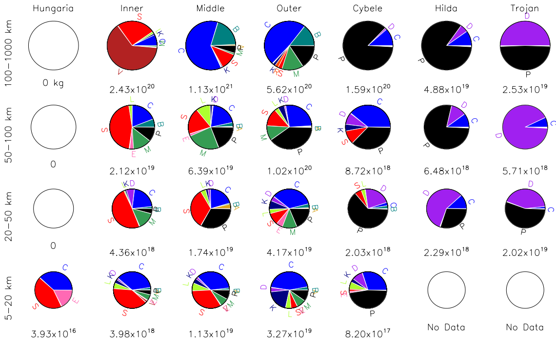
Fig 4. The compositional mass distribution as a function of size throughout the main belt out to the Trojans. The mass is calculated for each individual object with a diameter of 50km and greater using its albedo to determine size and the average density for that asteroids taxonomic class. For the smaller sizes we determine the fractional contribution of each class at each size and semi-major axis, and then apply that fraction to the distribution of all known asteroids from the Minor Planet Center including a correction for discovery incompleteness at the smallest sizes in the middle and outer belt 19 . Asteroid mass is grouped according to objects within four size ranges including diameters of 100-1000km, 50-100km, 20-50km, and 5-20km. Seven zones are defined as in Fig 1: Hungaria, Inner, Middle, and Outer Belt, Cybele, Hilda, and Trojan. The total mass of each zone at each size is labeled and the pie charts mark the fractional mass contribution of each unique spectral class of asteroid. The total mass of Hildas and Trojans are underestimated because of discovery incompleteness. The relative contribution of each class changes with both size and distance.
