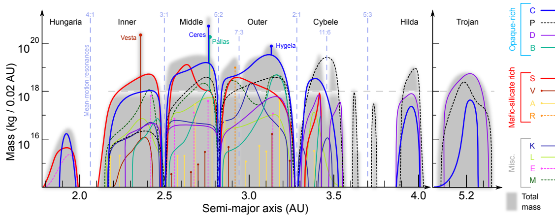
Fig 3. The compositional mass distribution throughout the asteroid belt out to the Trojans. The gray background is the total mass within each 0.02-au bin. Each color represents a unique spectral class of asteroid, denoted by a letter in the key. The horizontal line at 10^{18} kg is the limit of the work from the 1980s 2,8,9 . While the upper portion of the plot remains consistent with that work, immense detail is revealed at the lower mass range 19 .
