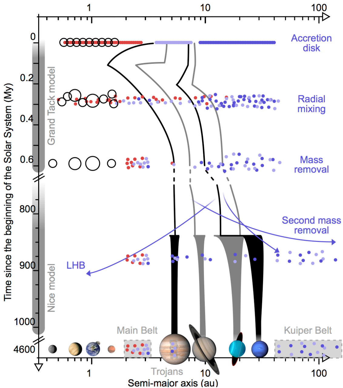
Fig 2. Cartoon of the effects of planetary migration on the asteroid belt. This figure captures some major components of the dynamical history of small bodies in the solar system based on models 11,12,50,53 . These models may not represent the actual history of the solar system, but are possible histories. They contain periods of radial mixing, mass removal, and planet migration-ultimately arriving at the current distribution of planets and small-body populations.
