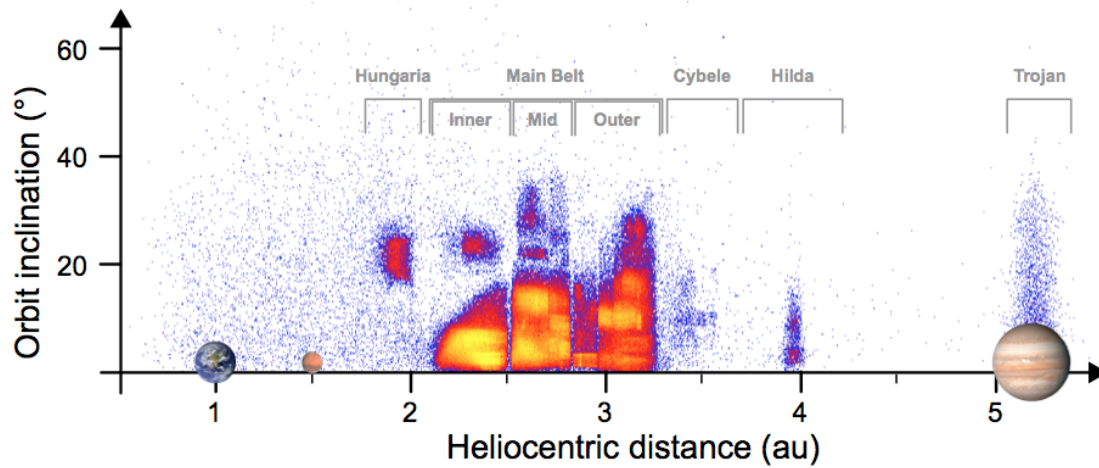
Fig. 1 The asteroid belt in context with the planets. This plot shows the location of the main belt with respect to the planets and the sun as well as the orbital structure of asteroid inclinations and number density of objects (yellow represents highest number density, blue the lowest). Asteroids have much higher orbital eccentricities and inclinations than do the planets. The structure of the belt is divided by unstable regions, seen most prominently at 2.5 and 2.8 au (locations where an asteroid's orbit is 'in resonance' with Jupiter's orbit), that separate the inner, middle, and outer sections of the main belt. The Hungaria asteroids are located closer to the Sun than is the main belt and have orbital inclinations centered near 20 degrees. The Hildas are located near 4 au and the Jupiter Trojans are in the L4 and L5 Lagrange points of Jupiter's orbit.
