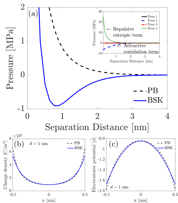
Figure 2. Disjoining pressures operating between two similarly charged surfaces separated by a 2:1 electrolyte solution predicted using the BSK model (eq 21) and the PB (eq 22) models for q_s = -0.1 C/m 2 , c_0 = 0.1 M, and \epsilon_r = 80 . (a) Variation of the disjoining pressure as a function of the separation distance between the two charged surfaces. The inset shows the contribution of the different terms in eq 21 based on the BSK model. (b,c) Comparison of the charge density and the dimensionless electrostatic potential profiles, respectively, predicted by the BSK model (eq 11) and the PB model (eq 11 with \delta_c set to zero) when the separation distance between the two charged surfaces is 1 nm, and where x is the spatial coordinate perpendicular to the plane of the charged surface.
