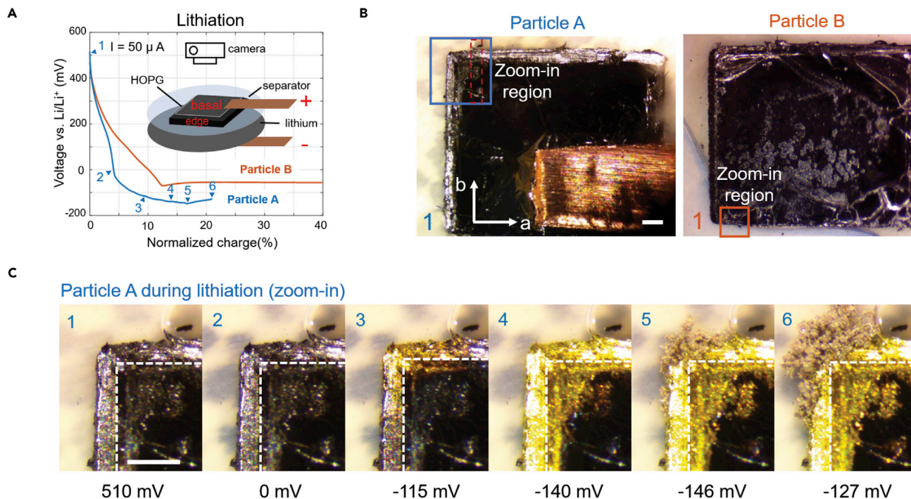
Figure 3. Voltage Profile and Optical Images during Lithiation
