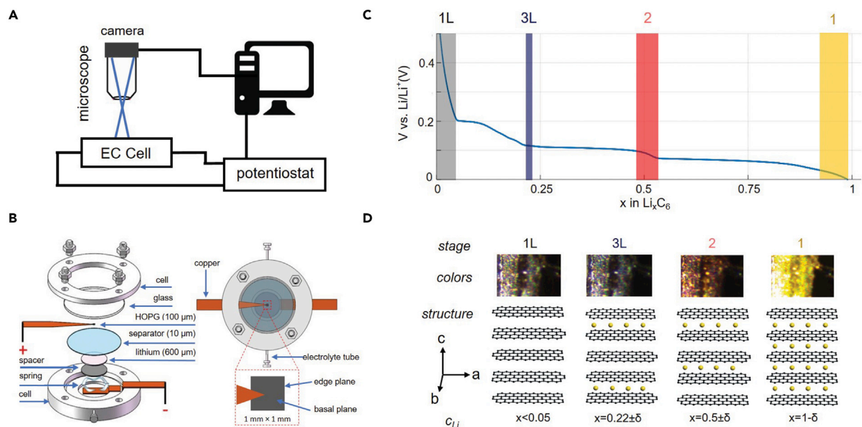
Figure 2. The Experimental Apparatus and Principle
