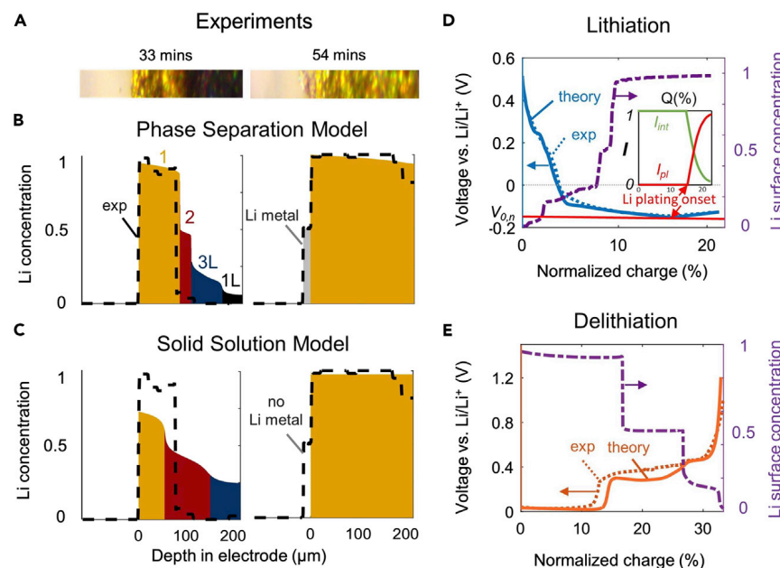
Figure 6. Theory and Simulation
