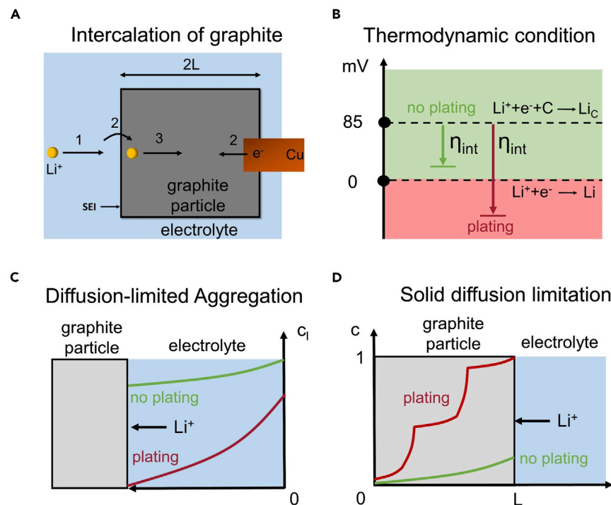
Figure 1. Proposed Mechanisms of Li Plating on Graphite
